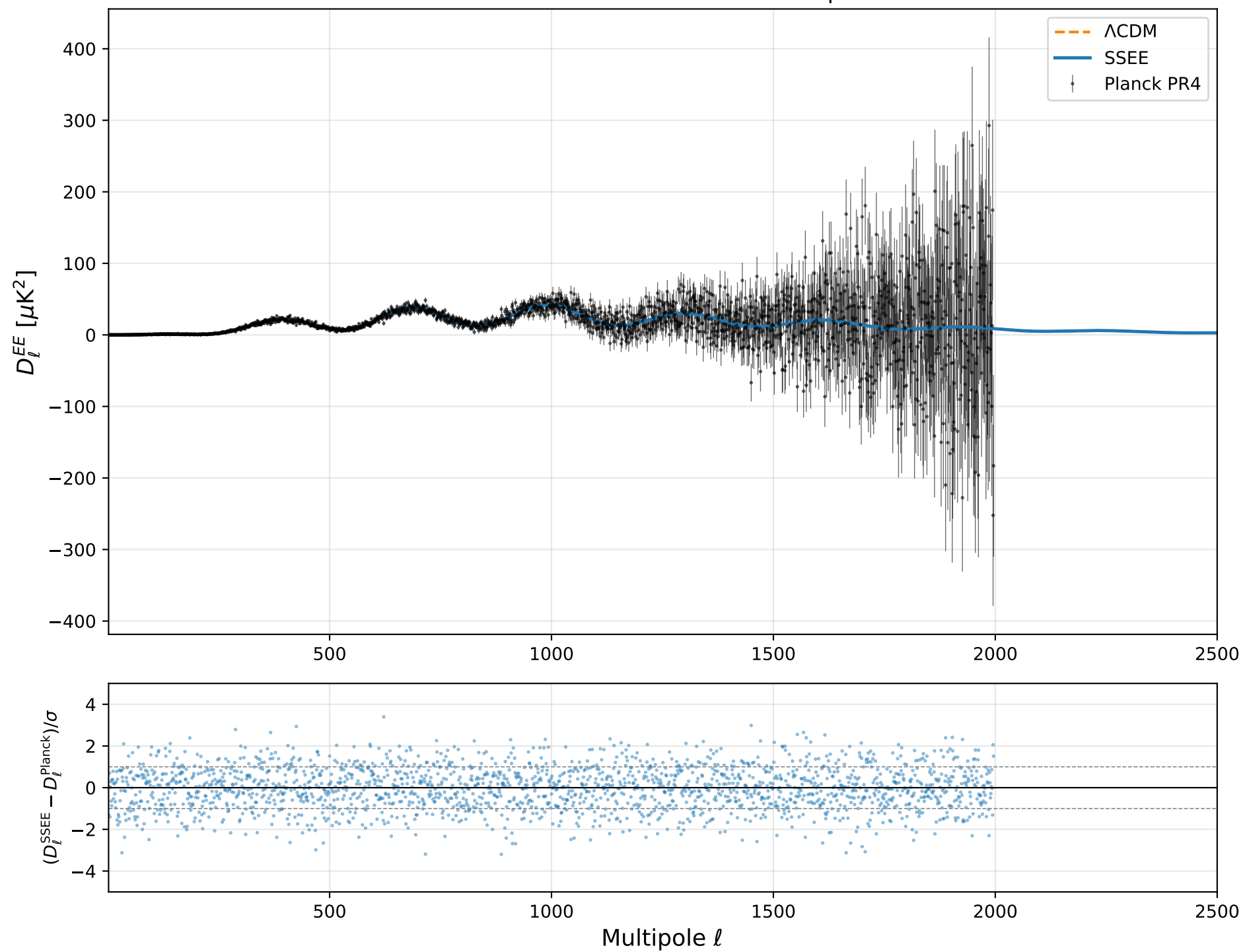
SSEE vs Planck PR4: CMB EE Power Spectrum
