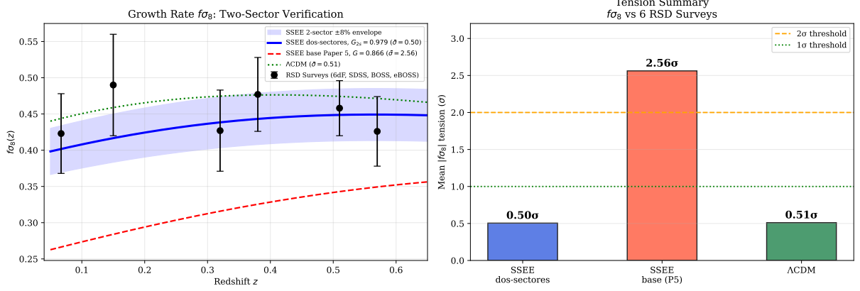
Figure 1: Left: f\sigma_8(z) predictions for the two-sector SSEE-V3.6 model (blue solid, mean 0.50\sigma ), SSEE-V3.6 Paper 5 base (red dashed, 2.56\sigma ), and \Lambda CDM (green dotted, 0.51\sigma ), compared to six RSD surveys (black points). Right: Mean |f\sigma_8| tension bar chart for the three models. Model parameters: G_{2s} = 0.979 , \sigma_8^{\text{eff}} = 0.794 , m_\phi = 5.71 eV.
