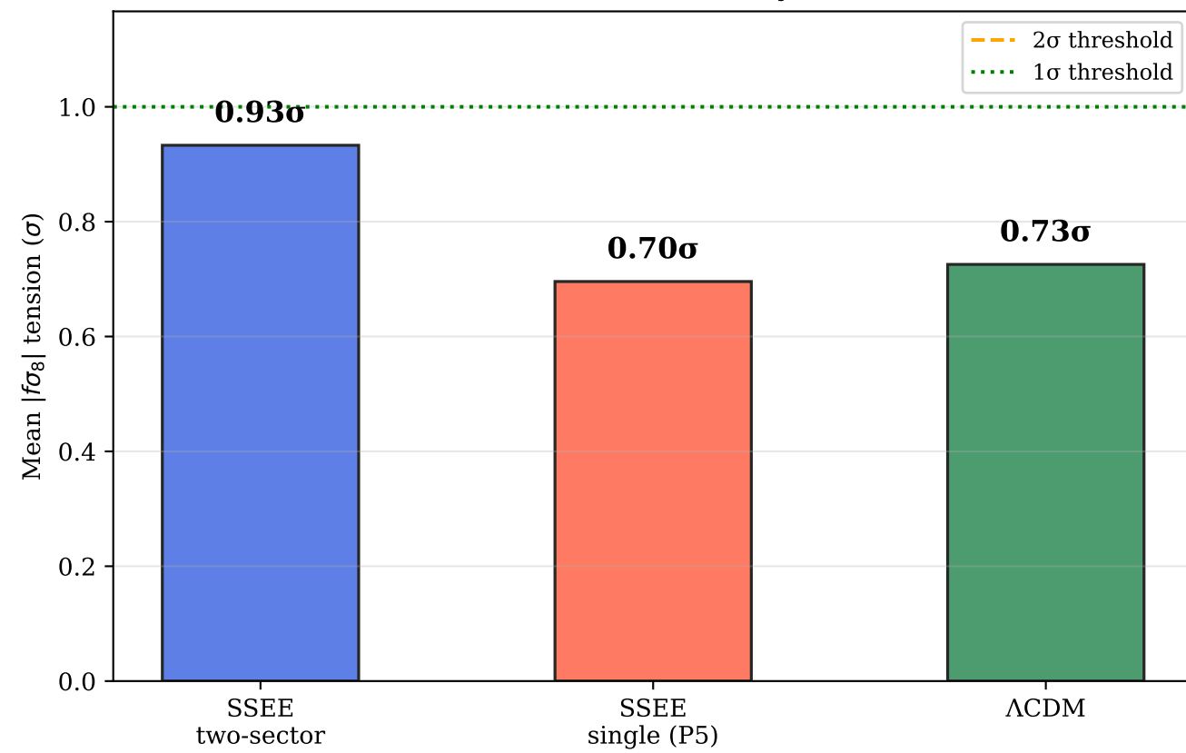
Tension Summary f\sigma_8 vs 6 RSD Surveys
