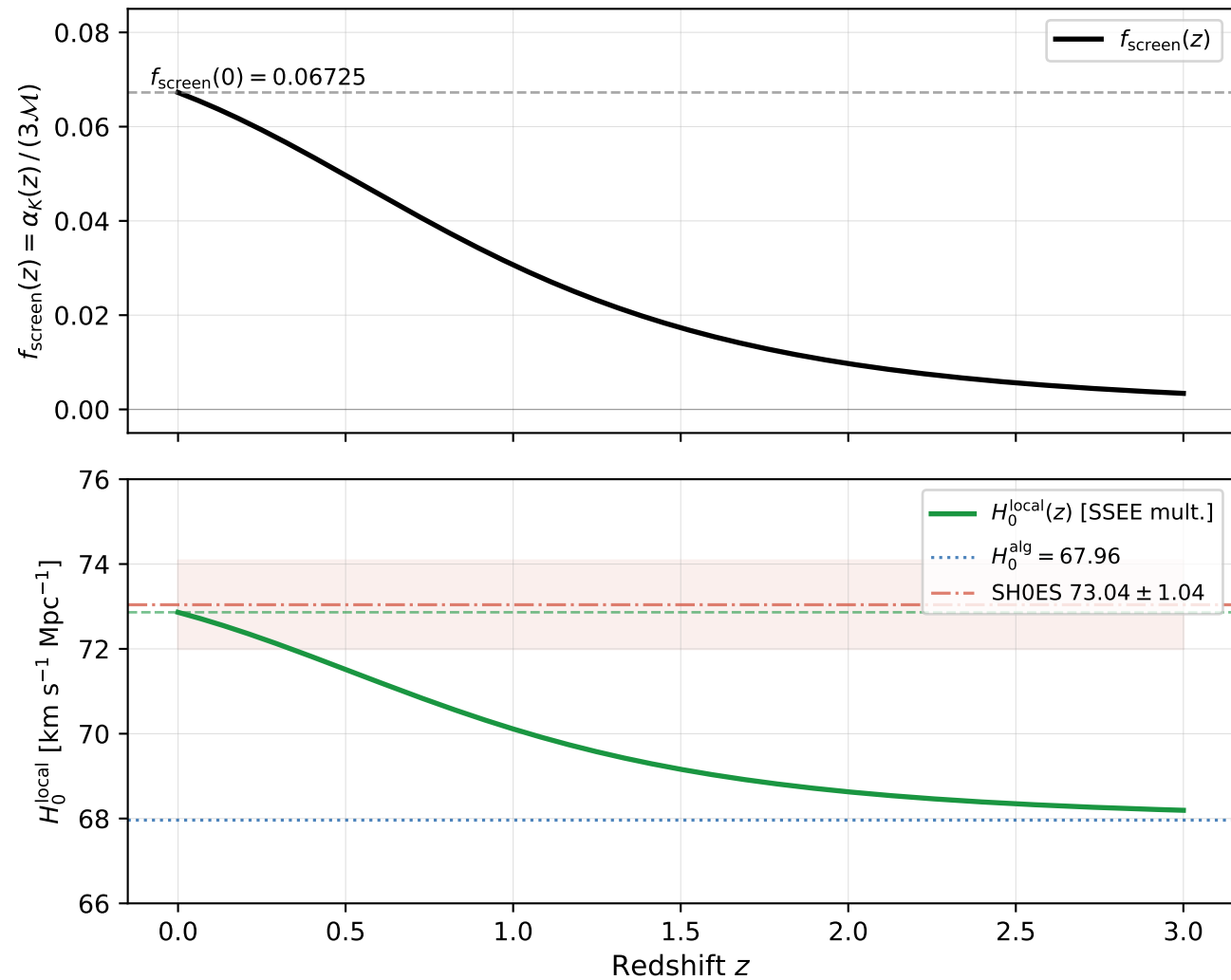
SSEE screening fraction and effective H_0 vs redshift
