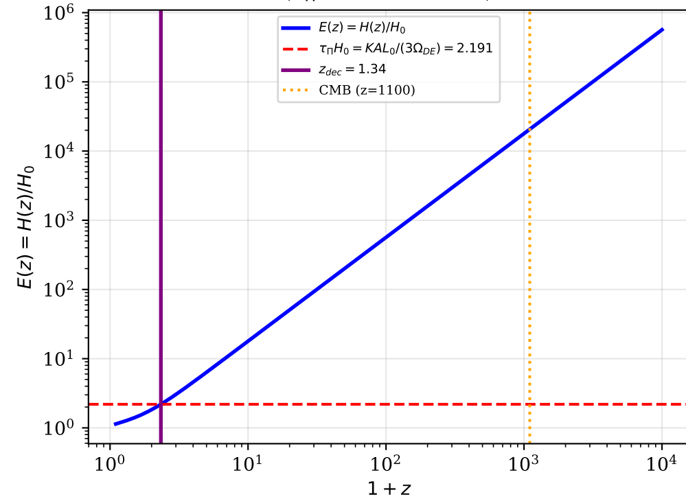
\phi -DM Decoupling Timeline (\tau_{\text{I}}H = 1 condition)
