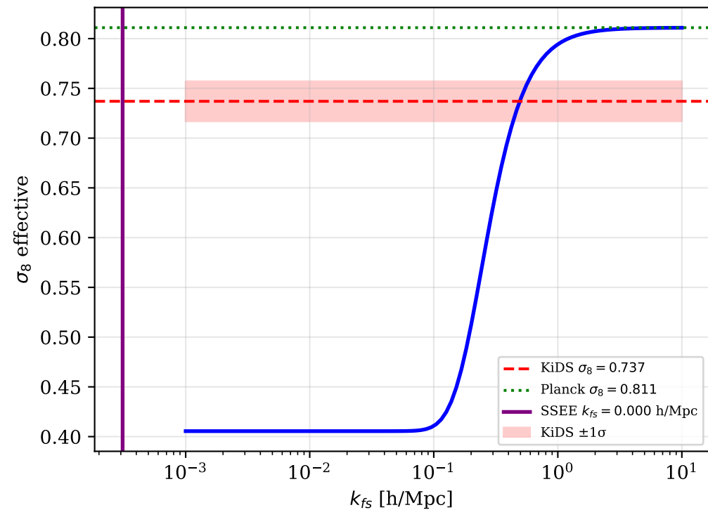
Two-Sector DM \sigma_8 vs free-streaming scale
