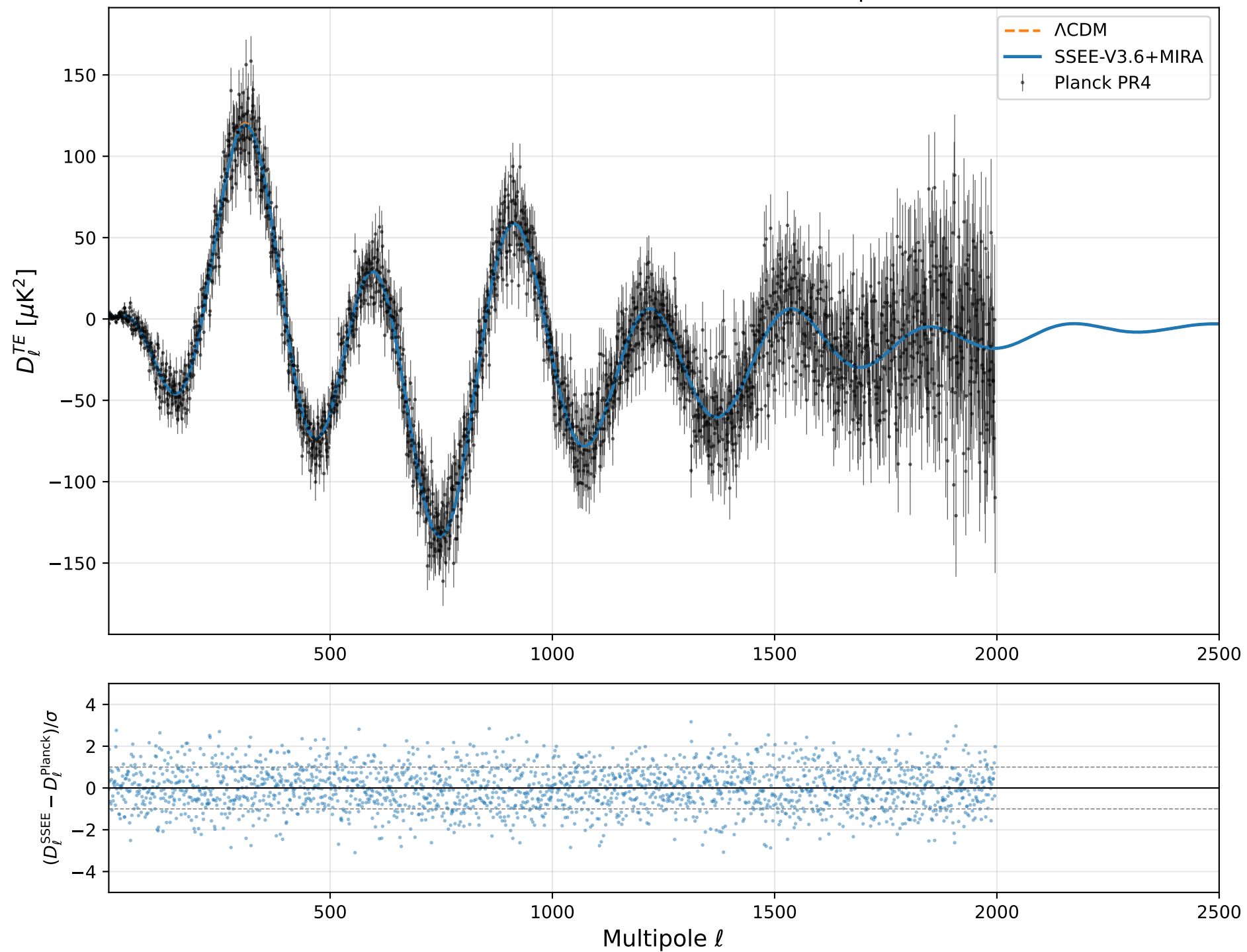
SSEE-V3.6 vs Planck PR4: CMB TE Power Spectrum
