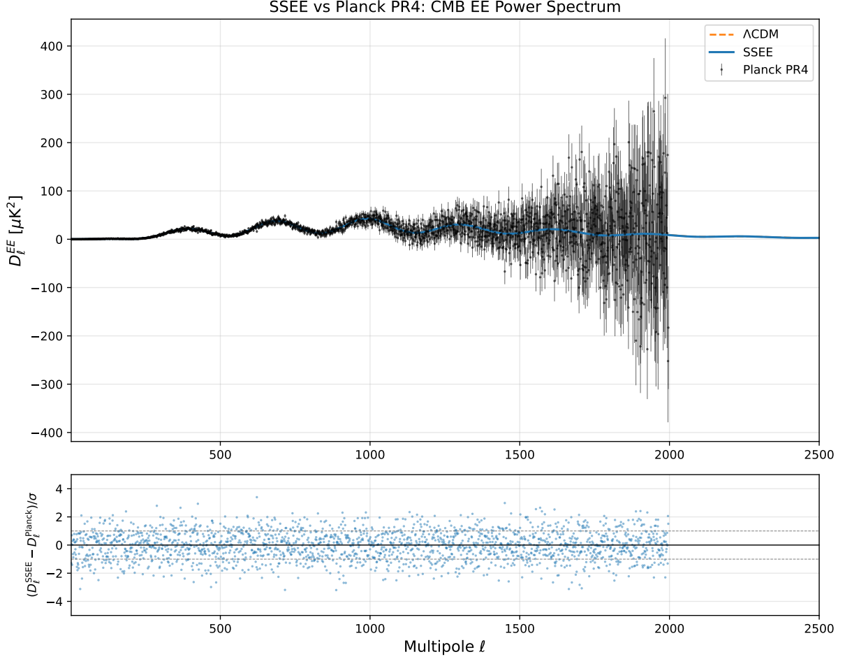
Figure 4: CMB EE polarization power spectrum D_\ell^{EE} [\mu\text{K}^2] . Blue: SSEE. Orange dashed: \Lambda CDM. Black points: Planck PR4 EE data.
