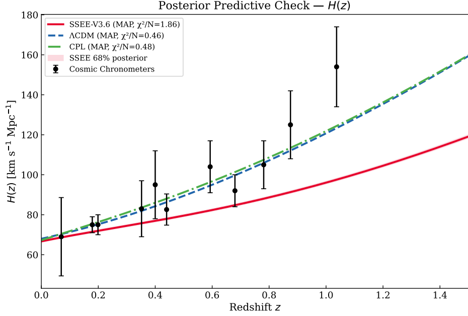
Figure 7: MAP H(z) vs Cosmic Chronometers (?). Red band: SSEE 68% posterior interval.
