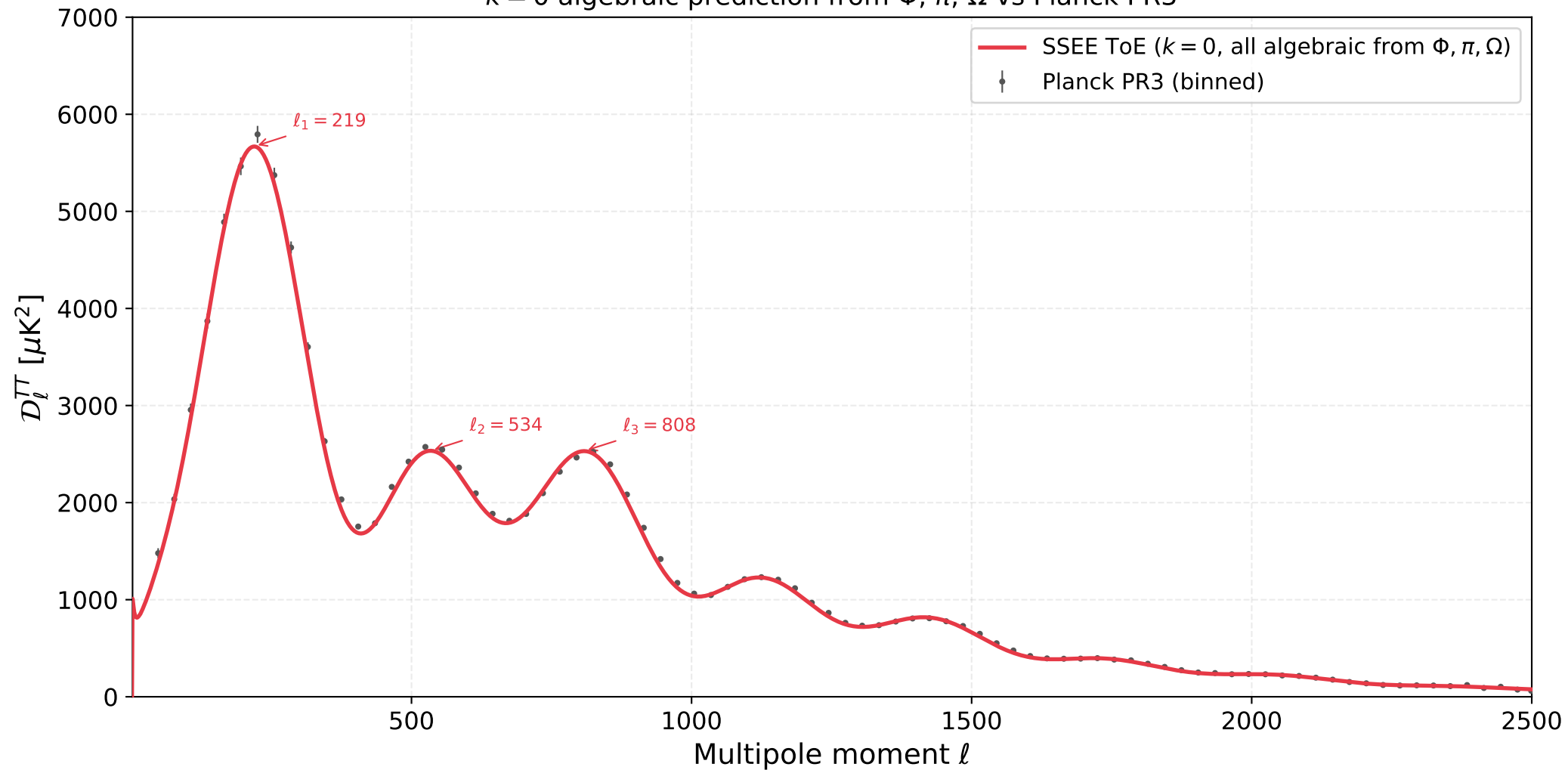
SSEE Theory of Everything: CMB Temperature Spectrum k = 0 algebraic prediction from \Phi, \pi, \Omega vs Planck PR3
