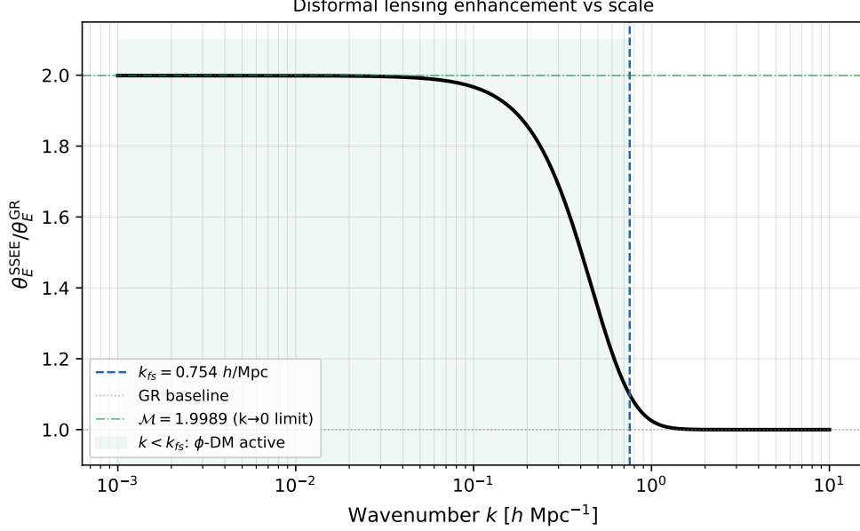
Figure 1: Disformal lensing enhancement \theta_E^{\text{SSEE}}/\theta_E^{\text{GR}} as a function of wavenumber k (h/Mpc). For k < k_{\text{fs}} = 0.754 \text{ h/Mpc} (blue dashed), the \phi -DM sector is active and the ratio approaches the algebraic limit \sqrt{\beta_c} = \sqrt{\mathcal{A}} \approx 1.9995 (dashed-dotted green), equivalent to \mathcal{M} = 1.999 . For k > k_{\text{fs}} the \phi -DM free-streams, the scalar gradient decouples, and lensing recovers the GR baseline (dotted). This is the pedagogical limit (a) (disformal scalar-force enhancement); the canonical limit (b) of the actual SSEE model recovers GR-with-DM lensing on all scales (Sec. 6.4).
