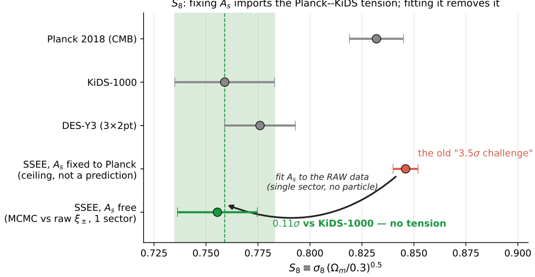
Figure 3: S_8 : fixing A_s imports the Planck–KiDS tension; fitting it removes it. The prediction of this paper with A_s held at the Planck value ( S_8 = 0.846 \pm 0.006 , red) sits 3.5\sigma above KiDS-1000 — but that offset is inherited from fixing A_s , not derived. Paper 6 (green) fits A_s to the raw shear data with the same background and a single matter sector, landing at S_8 = 0.7555 \pm 0.0192 — 0.11\sigma from KiDS-1000 (green band). Grey points: Planck 2018, KiDS-1000, and DES-Y3 measurements with 1\sigma errors.
