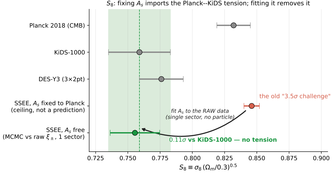
Figure 5: S_8 with the primordial amplitude fixed versus fitted. Red ( S_8 = 0.846 \pm 0.006 ): A_s held at the Planck value, which imports the Planck–KiDS discrepancy. Green ( S_8 = 0.755 \pm 0.0192 ): A_s fitted to the raw KiDS-1000 \xi_{\pm} data with a single matter sector and the background fixed by the algebra — 0.11\sigma from KiDS-1000 (green band). Grey points: Planck 2018, KiDS-1000 and DES-Y3 with 1\sigma errors. (An earlier version of this figure showed a two-sector \varphi -DM curve; that construction is retracted.)
