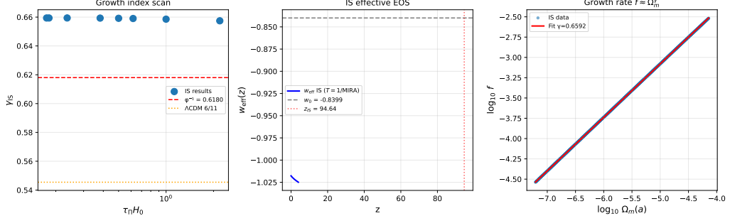
Figure 4: Israel-Stewart causal thermodynamics: prediction of the dynamical growth index and effective equation of state.
