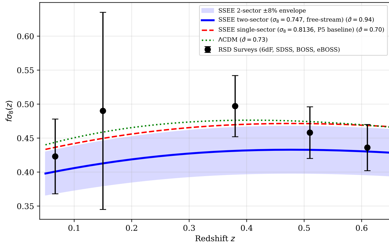
Growth Rate f\sigma_8 : Two-Sector Verification
