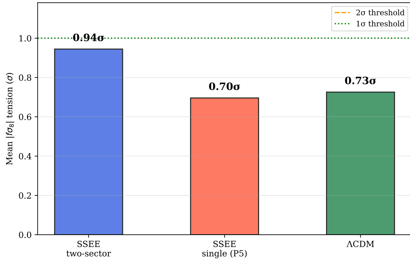
Tension Summary f\sigma_8 vs 6 RSD Surveys
