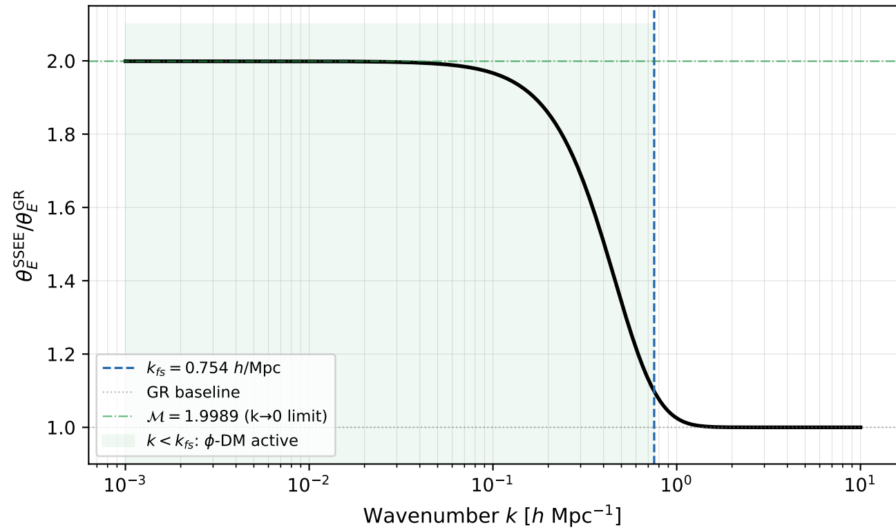
Disformal lensing enhancement vs scale
