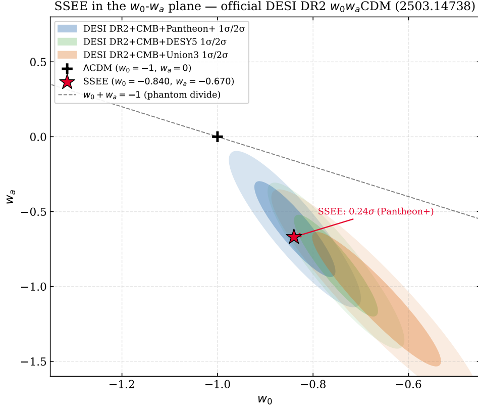
FIG. 1. The SSEE prediction in the w_0 - w_a plane. The single point (w_0, w_a) = (-T_r/M_v, -P_{sc}/\text{IGNIS}) = (-0.840, -0.670) is fixed entirely by \varphi and \pi , with no dark-energy parameters adjusted to the data. The shaded contours are the official DESI DR2 w_0w_a CDM posteriors (Pantheon+, DESY5, Union3). The SSEE point falls inside the Pantheon+ 1\sigma region; the joint Mahalanobis distance is \chi^2_{2D} = 0.42 , an equivalent 0.24\sigma agreement (Eq. 2), and within 1.5 – 1.8\sigma of the other compilations.
