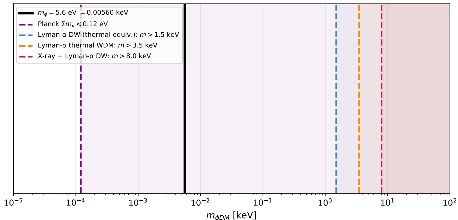
Route C — Mass exclusion limits
