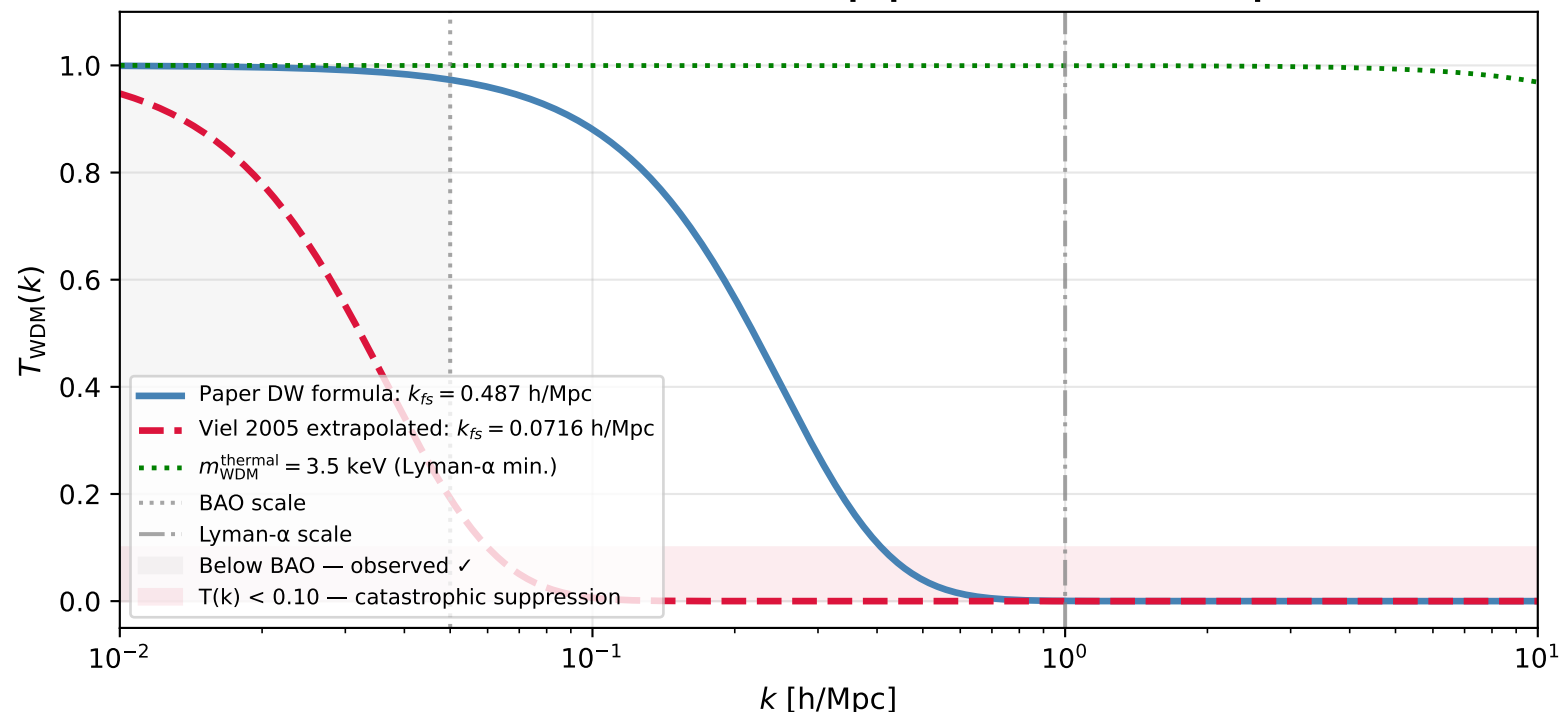
Route B — WDM transfer function: paper vs Viel 2005 extrapolation
