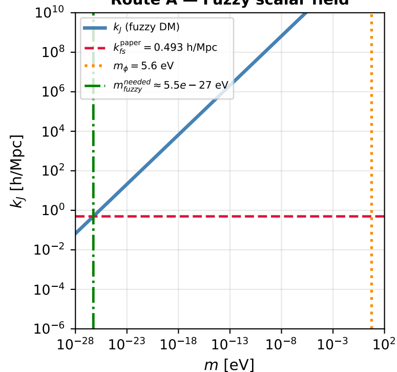
Route A — Fuzzy scalar field
