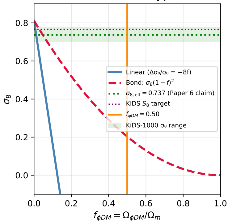
Route C — HDM \sigma_8 suppression
