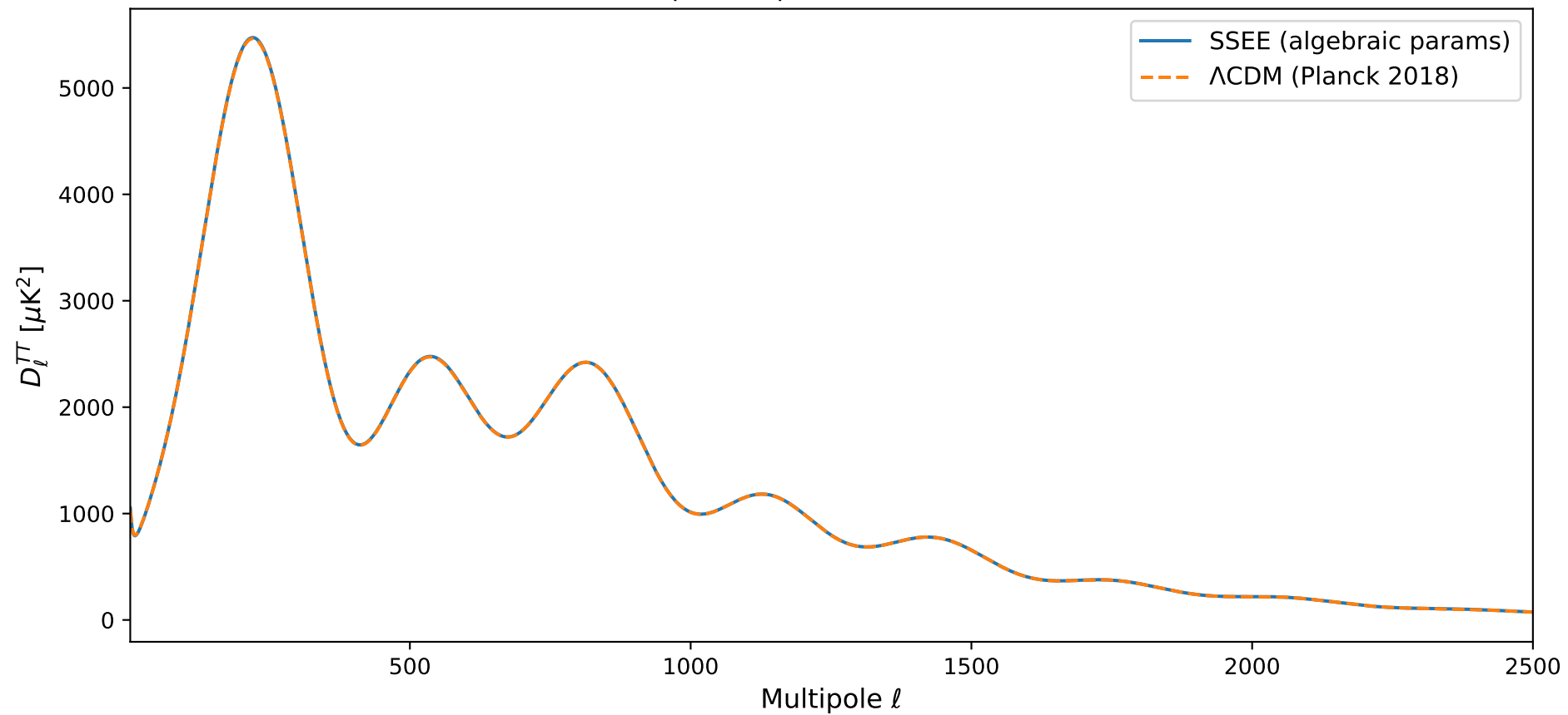
CMB TT power spectrum: SSEE vs \Lambda CDM
