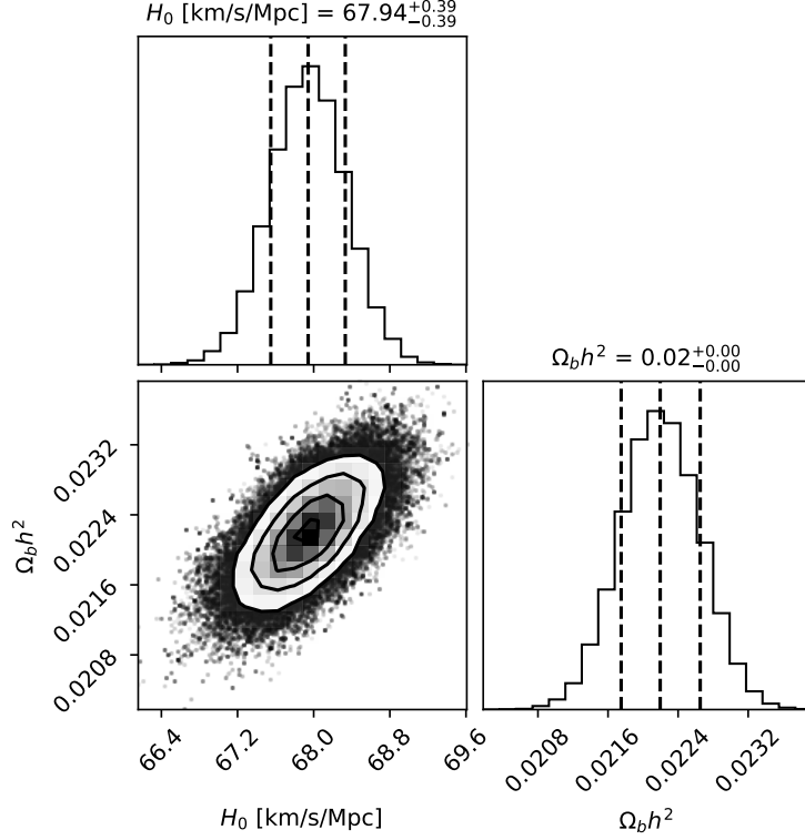
FIG. 3. Marginalised posterior from the MCMC analysis (100 walkers \times 25,000 steps). With the entire dark-energy sector fixed by \varphi and \pi , the chain samples only H_0 and \Omega_b h^2 against DESI DR2 BAO with the \omega_m -direct CMB anchor as prior. The posterior is H_0 = 67.9475 \pm 0.396 \text{ km s}^{-1} \text{ Mpc}^{-1} and \Omega_b h^2 = 0.02221 \pm 0.00045 (Eq. 8), coinciding with the anchor to 0.04\sigma . Dashed lines mark the anchor inputs ( H_0 = 67.962 \text{ km s}^{-1} \text{ Mpc}^{-1} , \Omega_b h^2 = 0.02218 ); the 16/50/84% quantiles are indicated.
