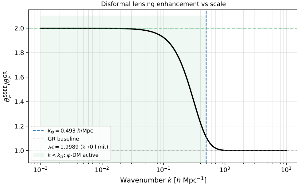
Figure 1: Disformal lensing enhancement \theta_E^{\text{SSEE}}/\theta_E^{\text{GR}} as a function of wavenumber k (h/Mpc). For k < k_{\text{fs}} = 0.493 \text{ h/Mpc} (blue dashed), the \phi -DM sector is active and the ratio approaches the algebraic limit \sqrt{\beta_c} = \sqrt{\mathcal{A}} \approx 1.9995 (dashed-dotted green), equivalent to \mathcal{M} = 1.999 . For k > k_{\text{fs}} the \phi -DM free-streams, the scalar gradient decouples, and lensing recovers the GR baseline (dotted).
