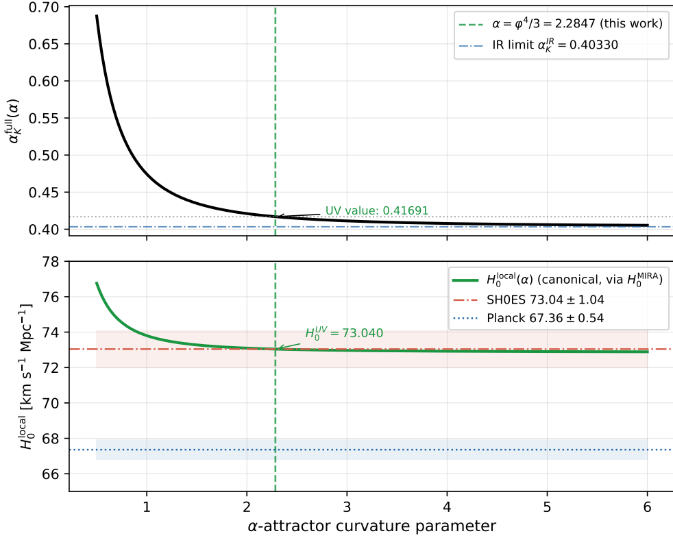
Figure 2: Top : Full Bellini–Sawicki parameter \alpha_K^{\text{full}}(\alpha) as the inflationary curvature \alpha varies. At \alpha = \varphi^4/3 = 2.284701 (green dashed), \alpha_K^{\text{full}} = 0.41691 (green dot); the IR limit 0.40330 is shown dash-dotted blue. Bottom : Predicted local Hubble constant H_0^{\text{local}}(\alpha) from the canonical cascade Eq. (21) with base H_0 = 67.962 km/s/Mpc (solid green), with the SH0ES band 73.04 \pm 1.04 km/s/Mpc (red) and Planck 67.36 \pm 0.54 km/s/Mpc (blue). If LiteBIRD measures r_{\text{obs}} , one reads off \alpha_{\text{obs}} = r_{\text{obs}} N^2/12 and the x -axis gives the falsifiable H_0 prediction. At \alpha = \varphi^4/3 the canonical value is 73.040 km/s/Mpc ( 0.00\sigma from SH0ES), inside the SH0ES band.
