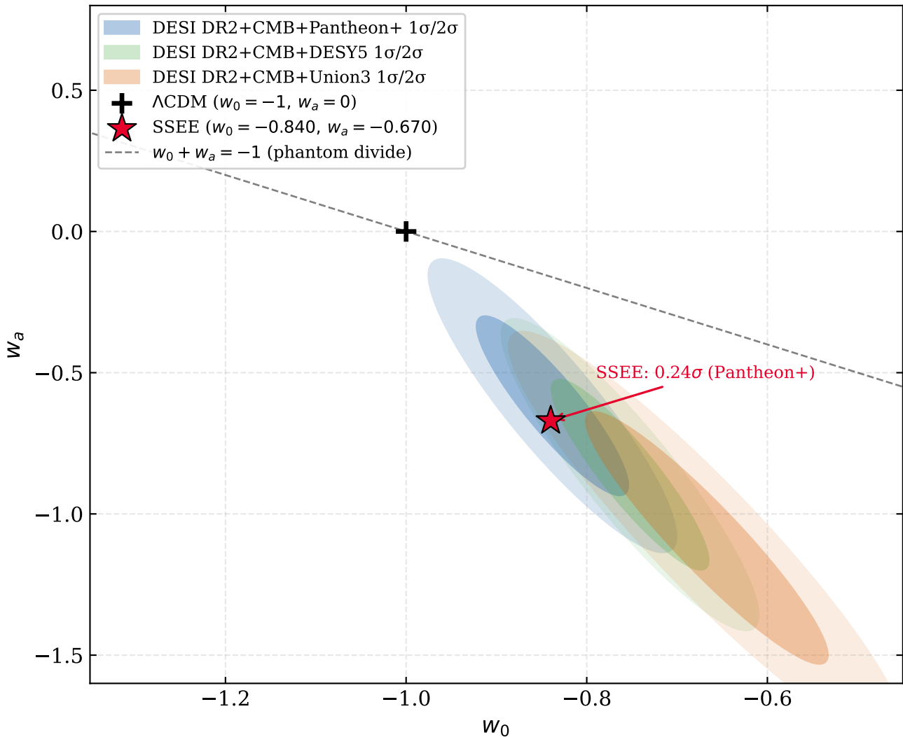
SSEE in the w_0 - w_a plane — official DESI DR2 w_0w_a CDM (2503.14738)
