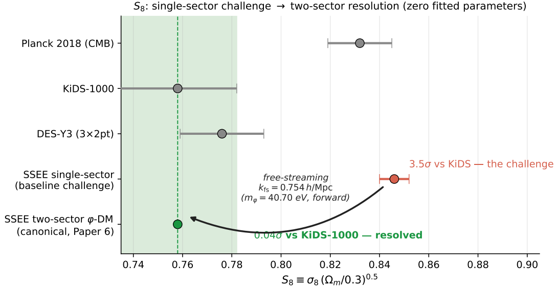
Figure 5: S_8 : the single-sector challenge and the two-sector resolution. The single-sector ceiling (red, S_8 = 0.846 \pm 0.006 ) carries the 3.5\sigma tension with KiDS-1000 reported in Eq. (14); the two-sector \varphi -DM extension (green, S_8 = 0.758 ) lands 0.04\sigma from KiDS-1000 (green band), with the free-streaming scale fixed by the forward-predicted mass m_\varphi = 40.70 \text{ eV} — no parameter fitted to lensing data. Grey points: Planck 2018, KiDS-1000 and DES-Y3 with 1\sigma errors.
