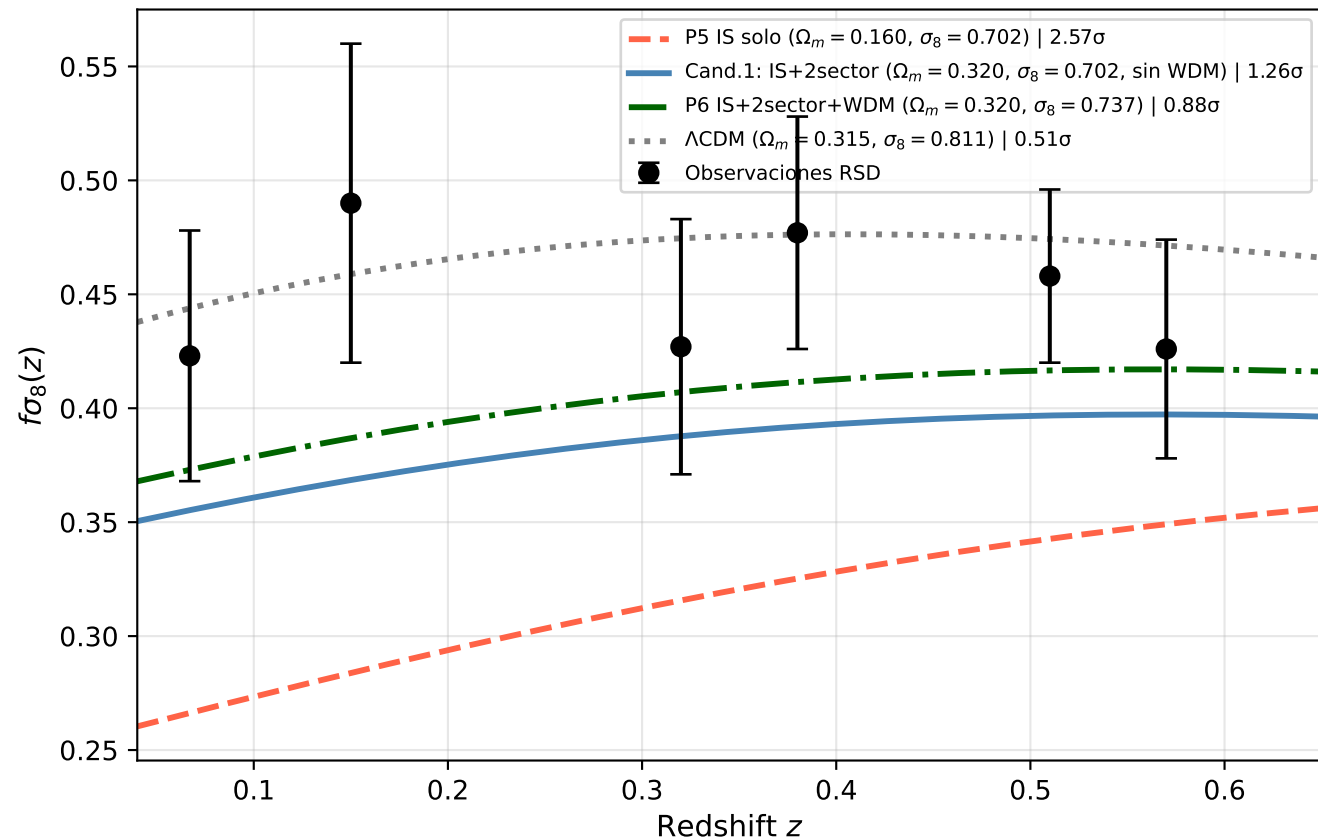
f\sigma_8 : IS solo vs IS+WDM
