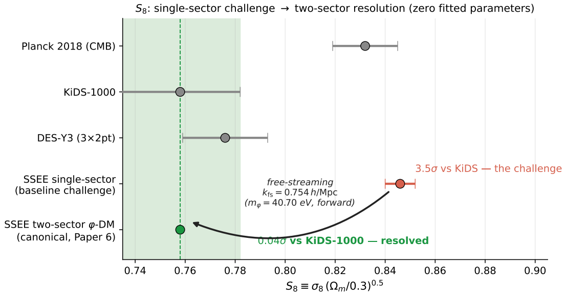
FIG. 5. S_8 : the single-sector challenge and the two-sector resolution. The single-sector ceiling (red, S_8 = 0.846 \pm 0.006 ) carries the 3.5\sigma tension with KiDS-1000 reported in Eq. (15); the two-sector \varphi -DM extension (green, S_8 = 0.758 ) lands 0.04\sigma from KiDS-1000 (green band), with the free-streaming scale fixed by the forward-predicted mass m_\varphi = 40.70 \text{ eV} — no parameter fitted to lensing data. Grey points: Planck 2018, KiDS-1000 and DES-Y3 with 1\sigma errors.
