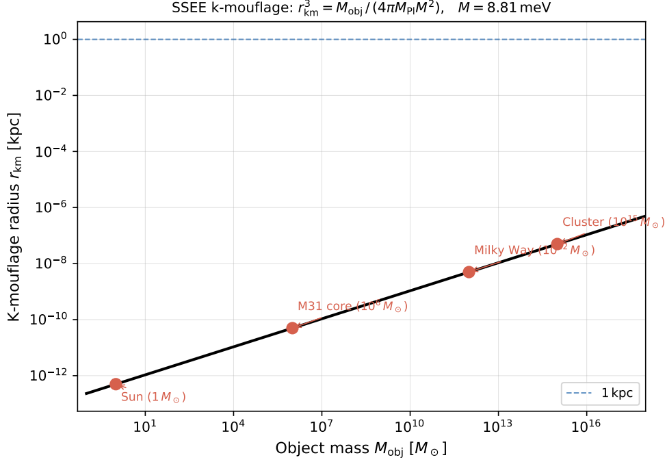
Figure 2: K-mouflage screening radius r_{\text{km}} = [M_{\text{obj}} / (4\pi M_{\text{Pl}} M^2)]^{1/3} as a function of object mass (in M_{\odot} ) at the UV completion scale M = 8.81 \text{ meV} (?). For all representative objects, r_{\text{km}} lies far below the galactic scale, so DM fifth-force dynamics are active at cosmological radii while baryons remain decoupled through selective coupling (Section ??).
