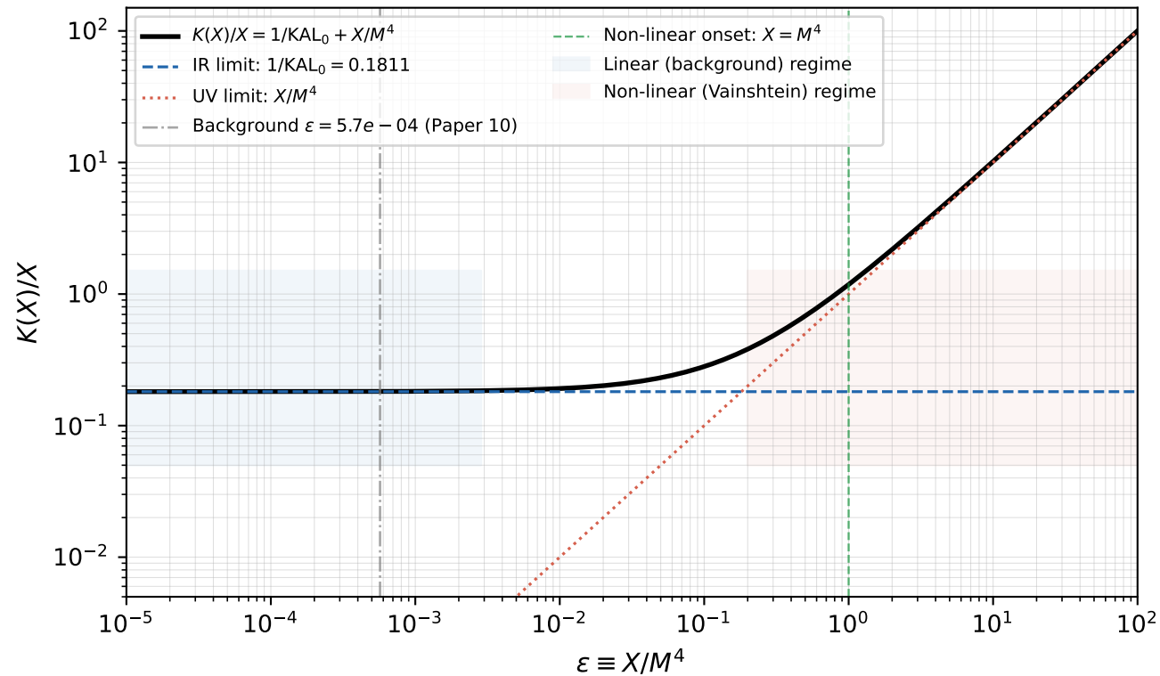
SSEE kinetic function K(X) = X/KAL_0 + X^2/M^4 : IR \rightarrow UV crossover
