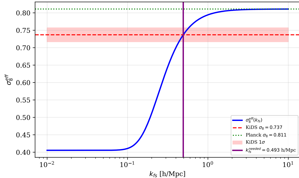
Two-Sector \phi -DM: \sigma_8 vs Free-streaming Scale
