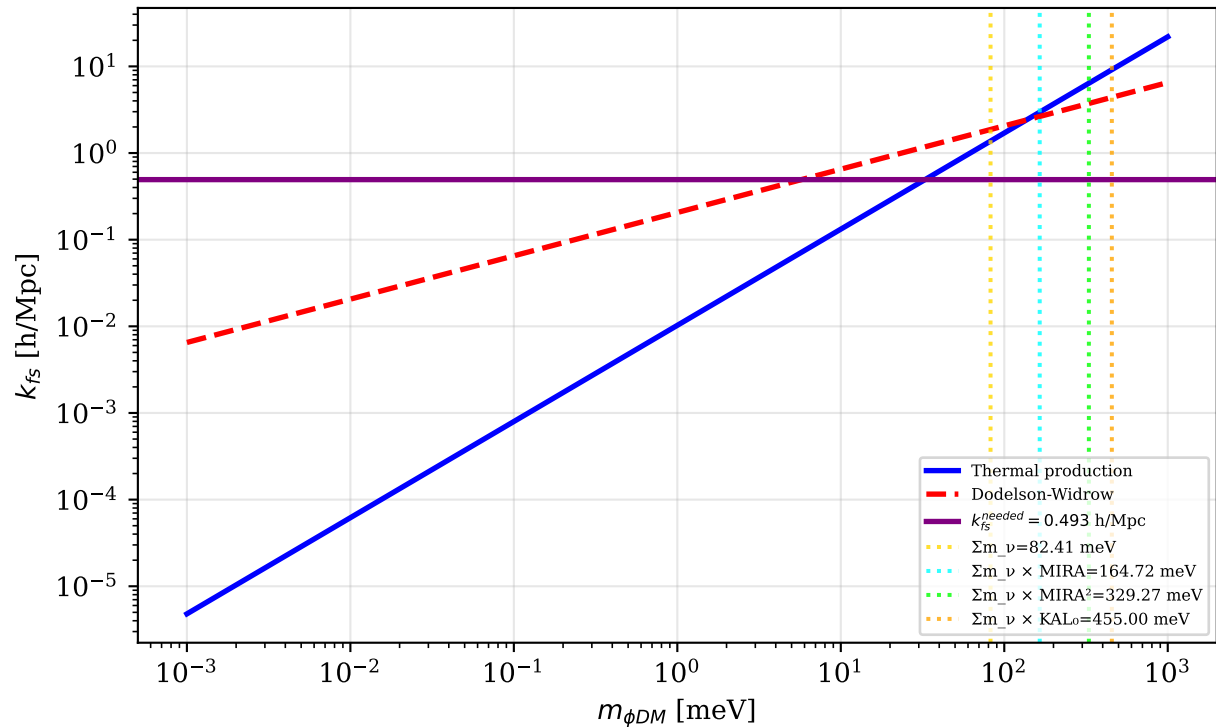
\phi -DM Mass \rightarrow Free-streaming Scale
