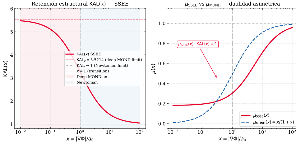
Figure 2: \text{KAL}(x) interpolation between the Newtonian limit ( x \gg 1 ) and the MONDian limit ( x \ll 1 ). The fixed point \text{KAL}_0 \approx 5.521 marks the structural retention at x = 0 , which enters both the cluster mass formula (5) and the acoustic-scale mapping hypothesis (6) (Section 2.4).
