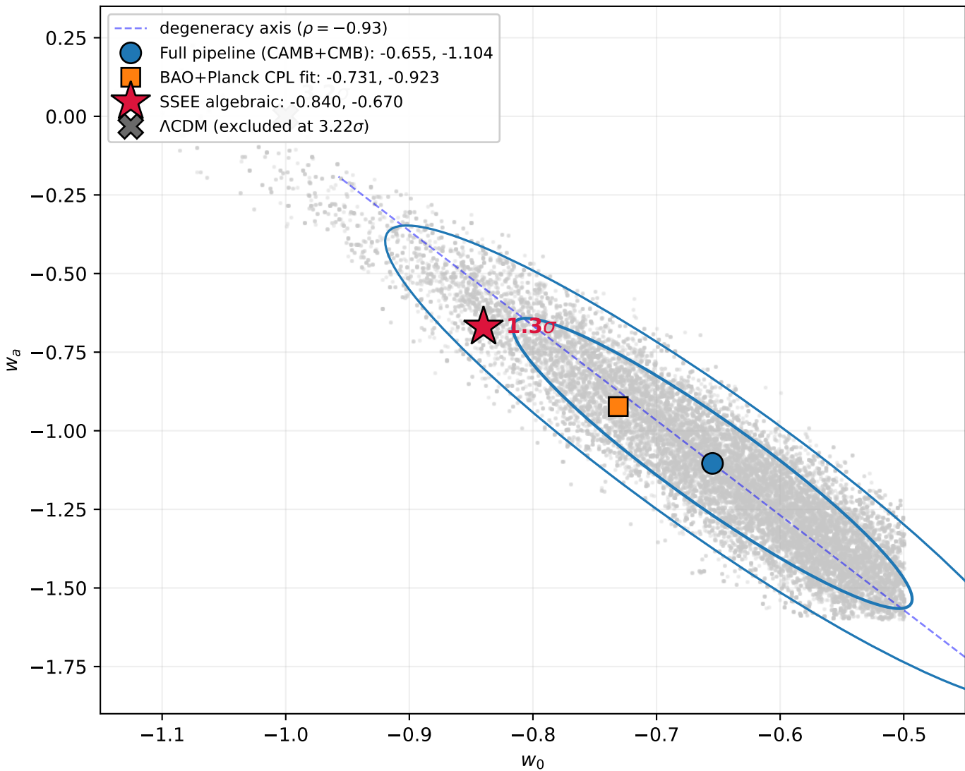
Full-likelihood w_0 - w_a posterior: SSEE lies within the data-preferred region
