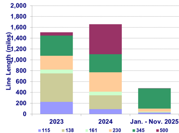
New Transmission Projects by Voltage
