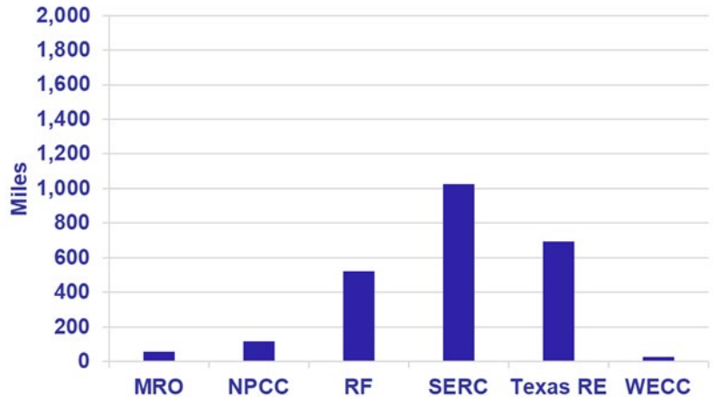
Transmission Projects with a High Probability of being completed by April 2028
