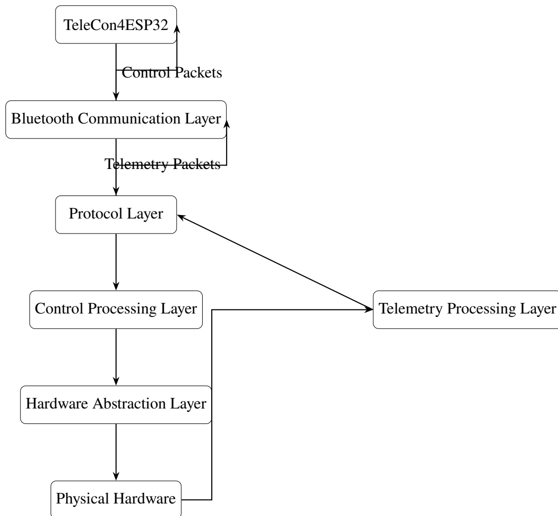
Figura 1.1: High-level system architecture and bidirectional data flow.
