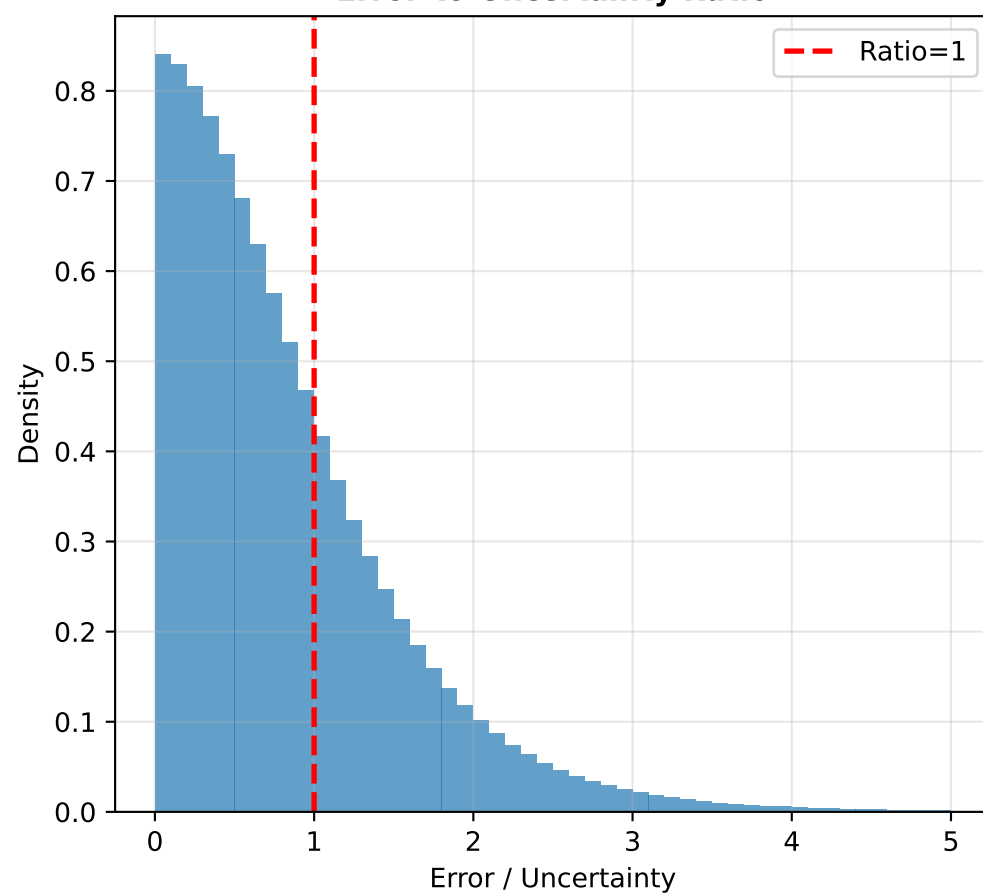
Error-to-Uncertainty Ratio
