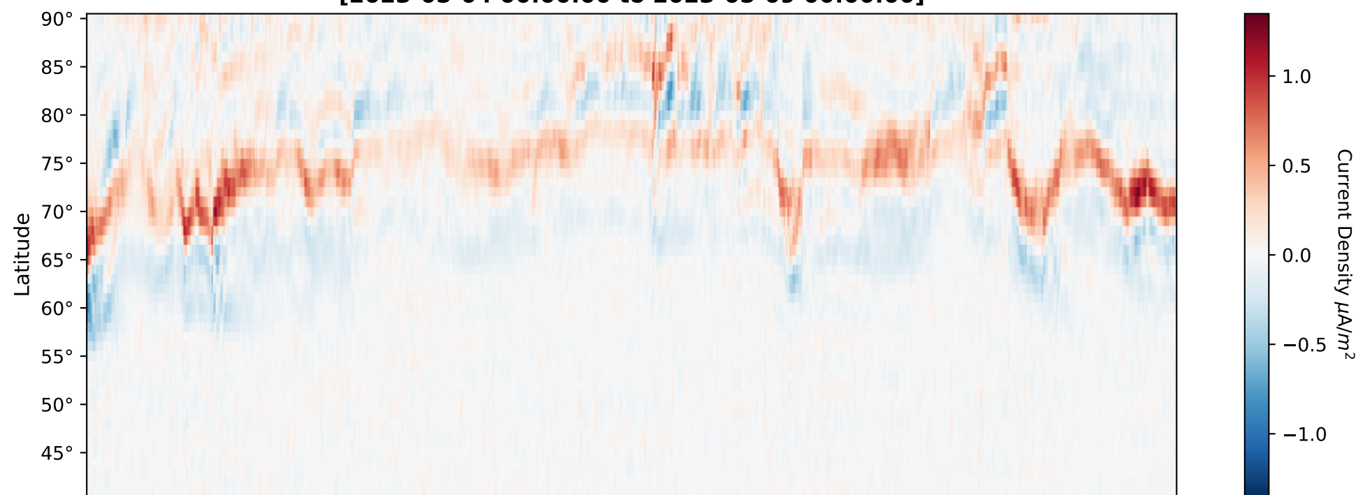
Predicted Data (MLT 15-21 avg)
