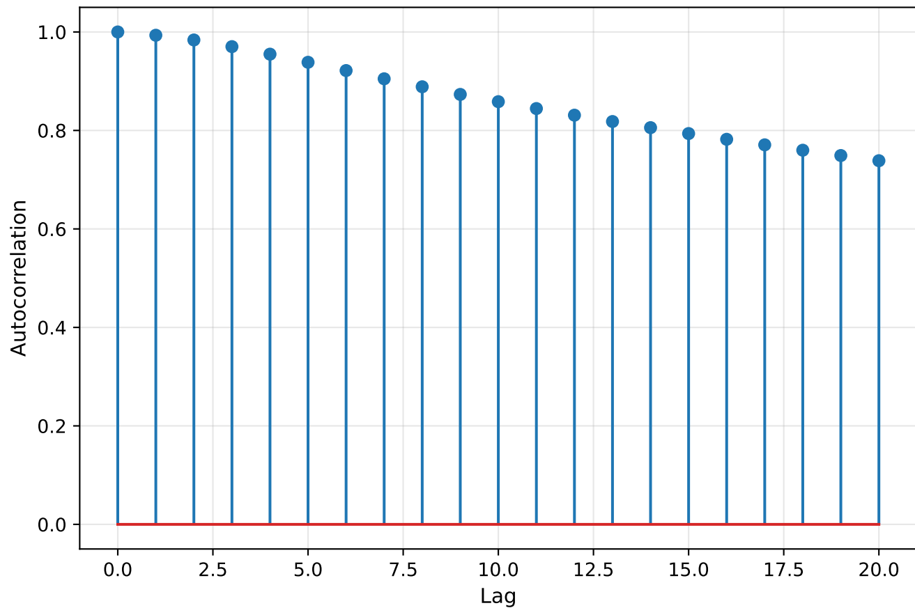
Predicted Autocorrelation (Lat 75-85°, MLT 15-21)
