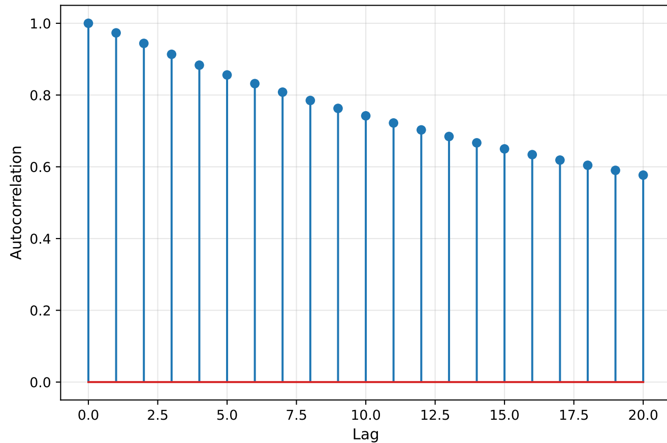
AMPERE Autocorrelation (Lat 75-85°, MLT 15-21)
