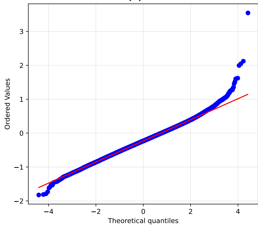
Q-Q Plot
