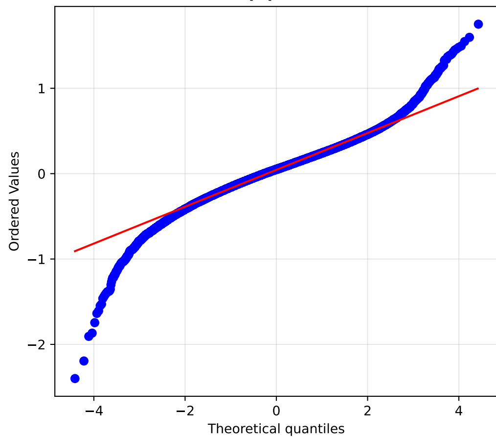
Q-Q Plot
