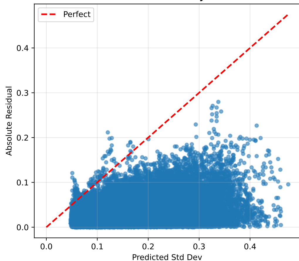
Calibration Curve
