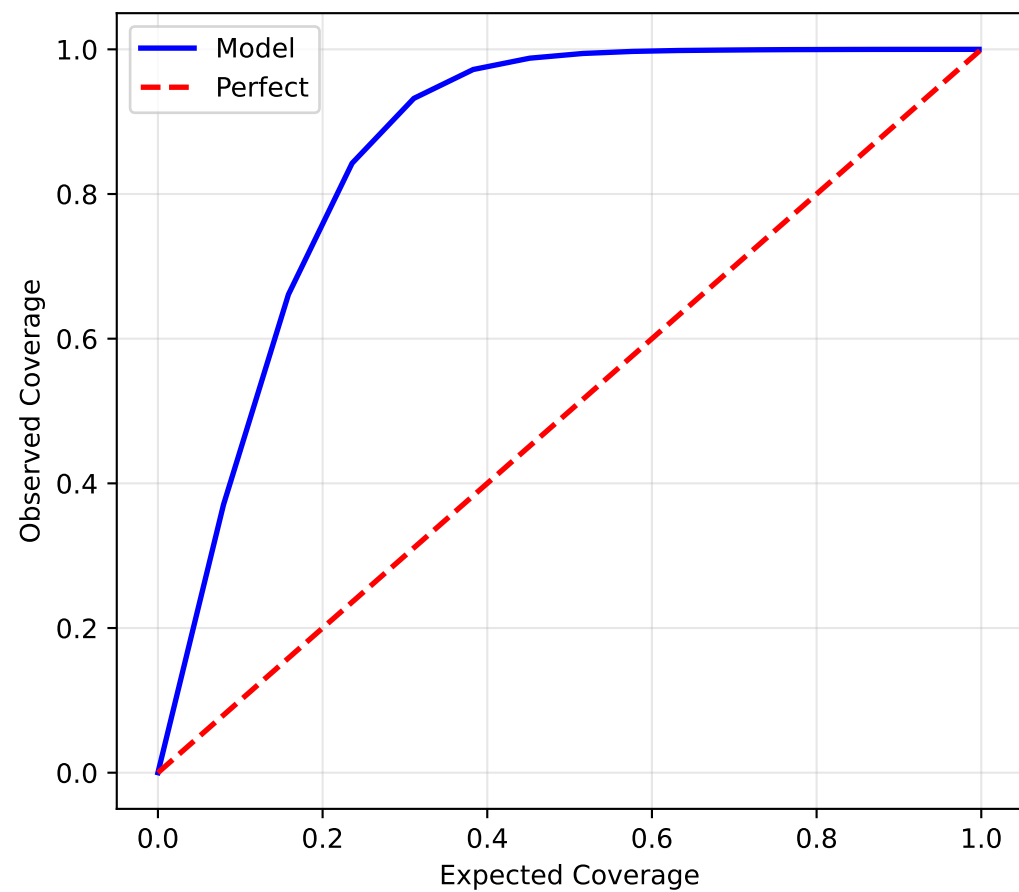
Calibration Curve
