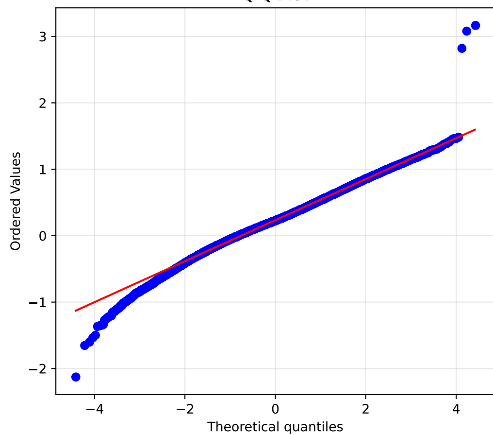
Q-Q Plot
