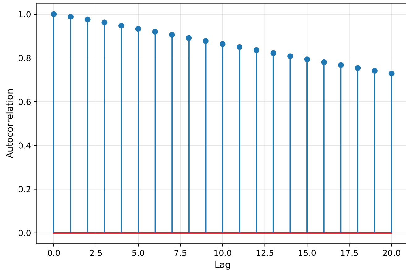
AMPERE Autocorrelation (Lat 65-75°, MLT 15-21)
