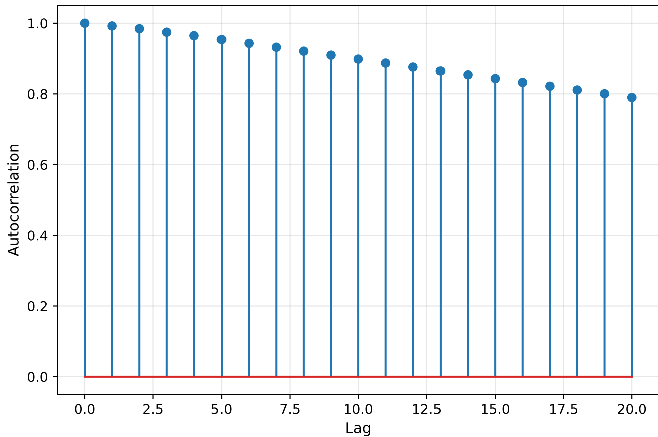
Predicted Autocorrelation (Lat 65-75°, MLT 15-21)
