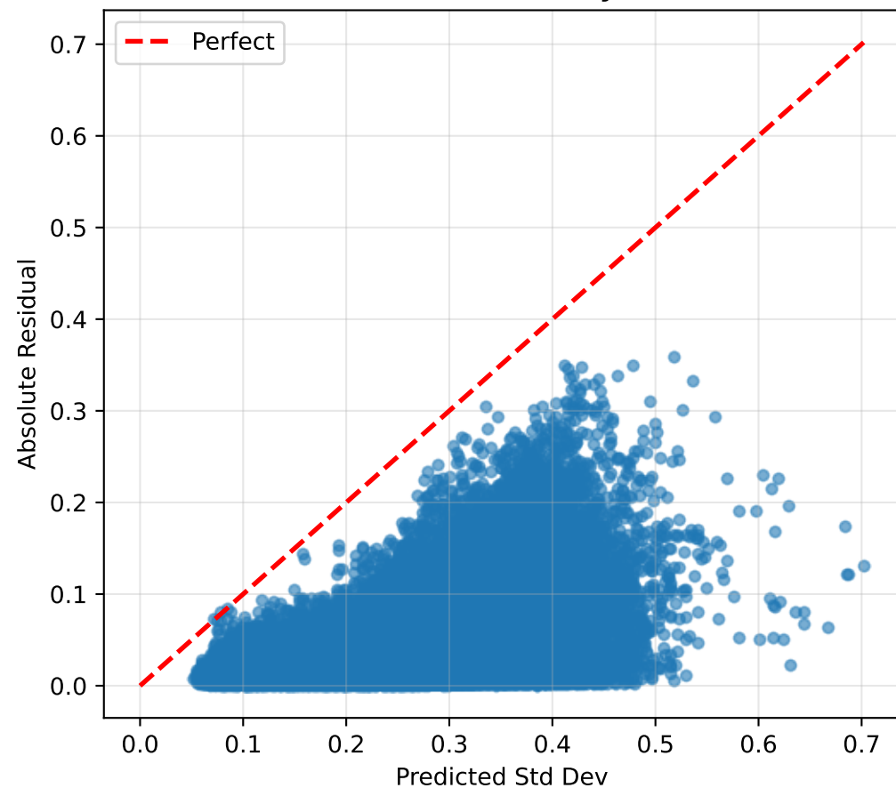
Calibration Curve
