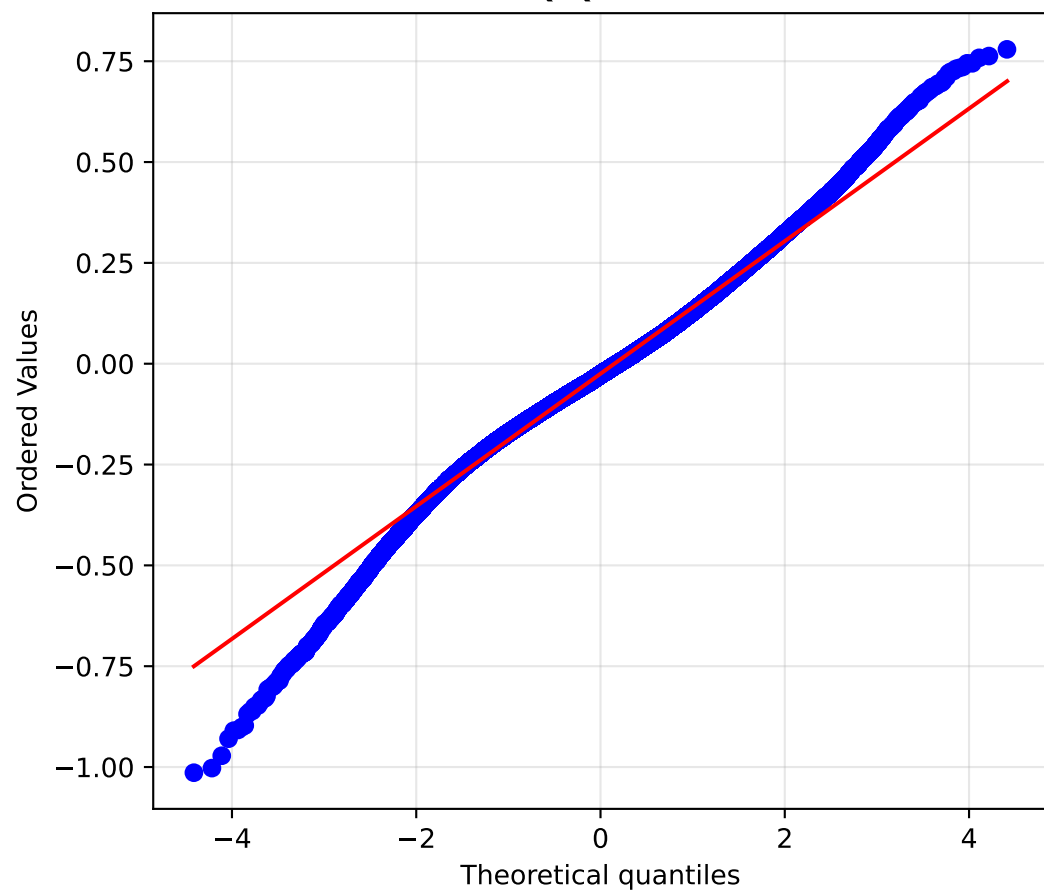
Q-Q Plot
