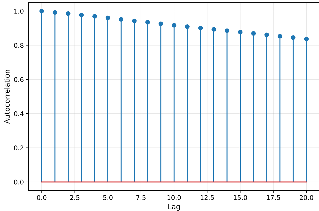
Predicted Autocorrelation (Lat 65-75°, MLT 21-3)
