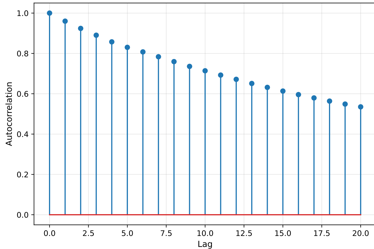
AMPERE Autocorrelation (Lat 65-75°, MLT 21-3)
