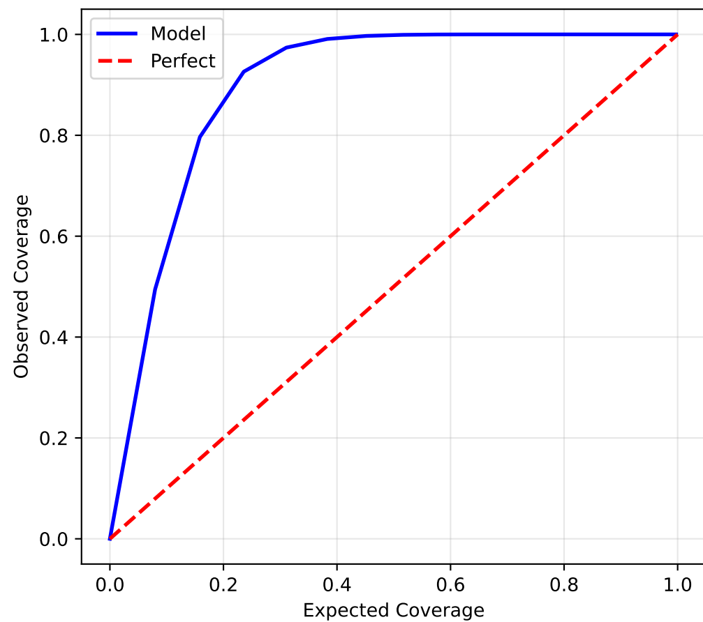
Calibration Curve
