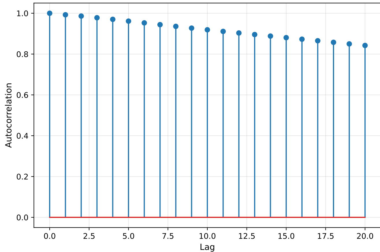
Predicted Autocorrelation (Lat 65-75°, MLT 22-2)
