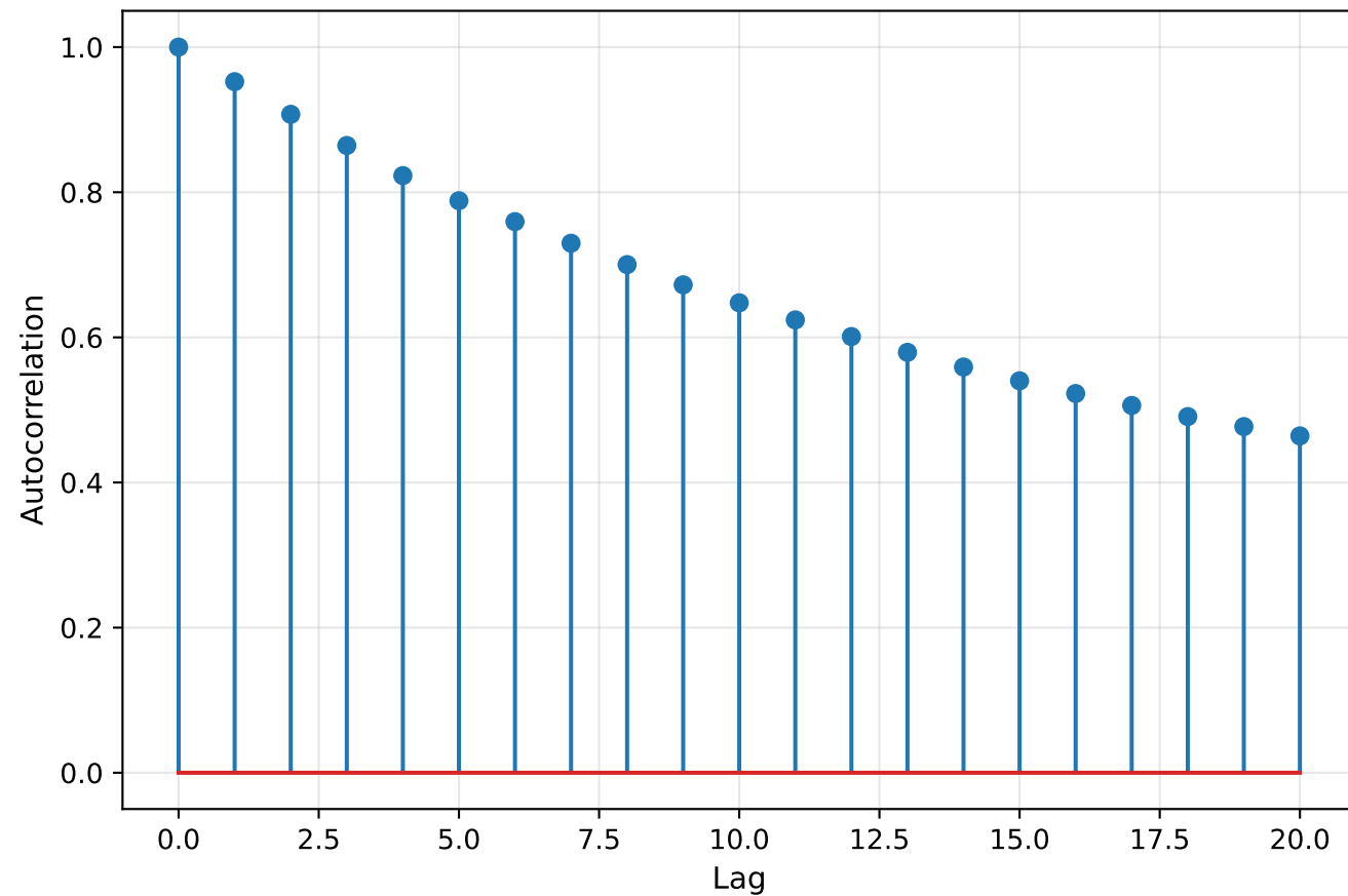
AMPERE Autocorrelation (Lat 65-75°, MLT 22-2)
