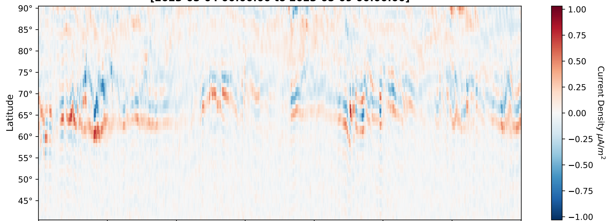
Predicted Data (MLT 22-2 avg)
