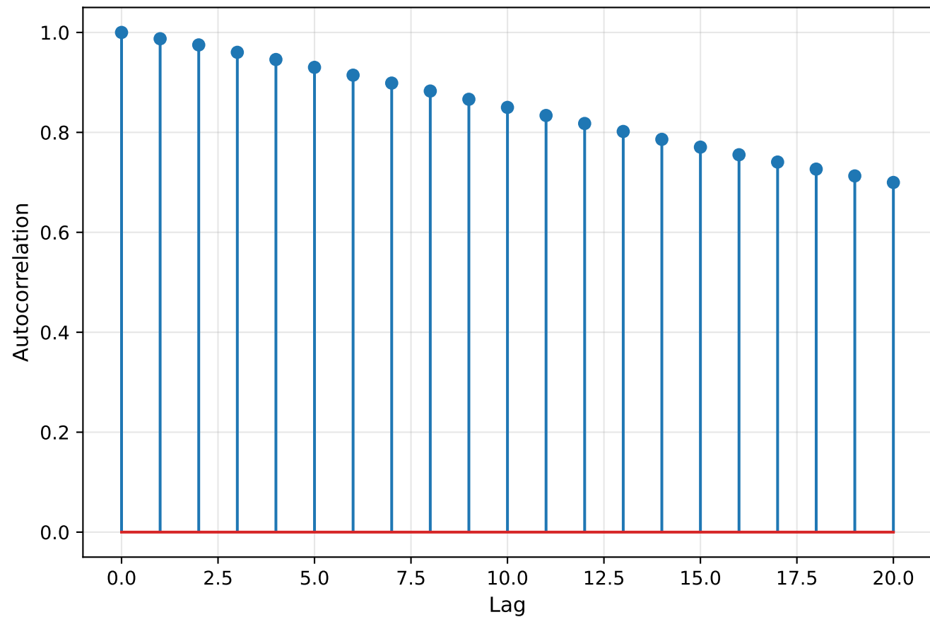
Predicted Autocorrelation (Lat 65-75°, MLT 3-9)
