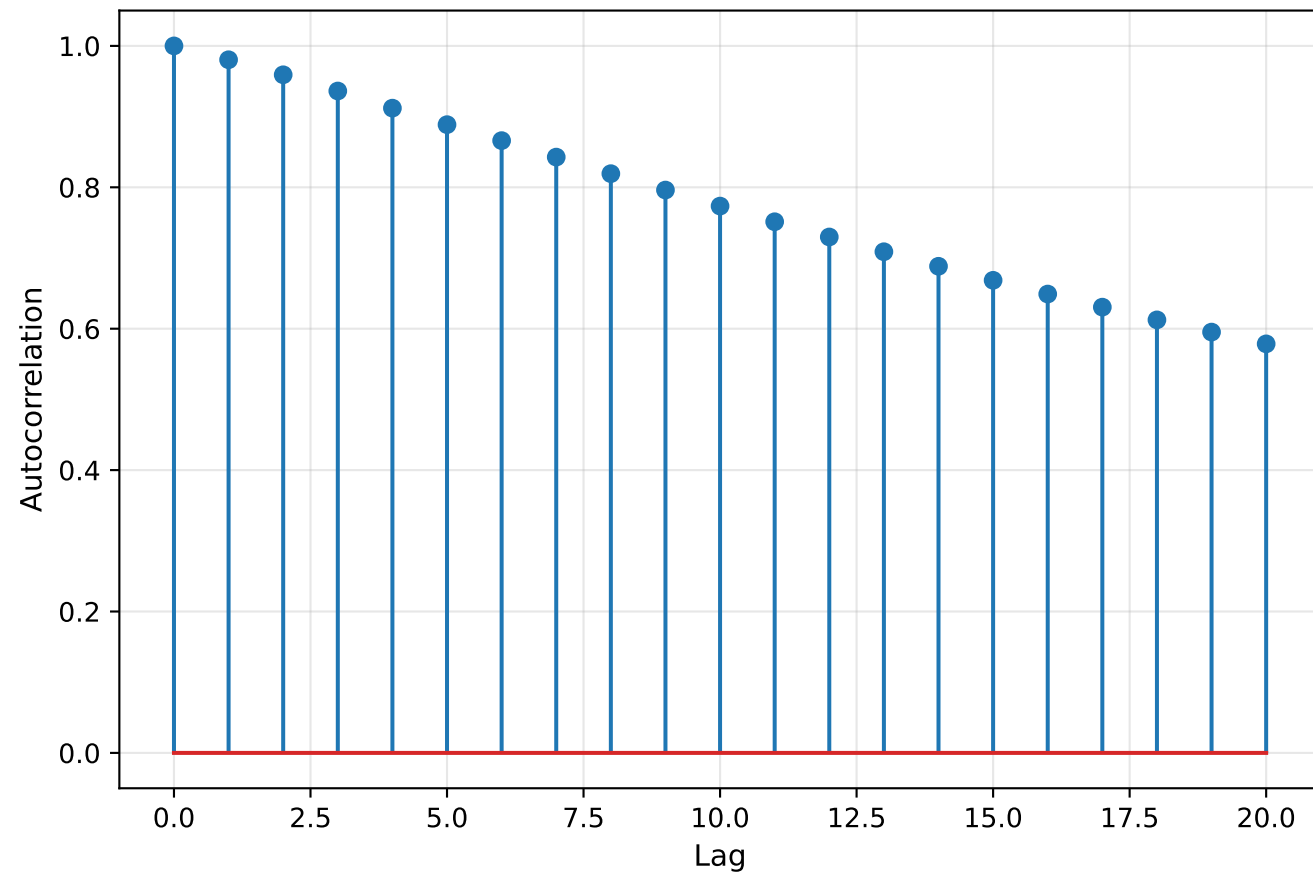
AMPERE Autocorrelation (Lat 65-75°, MLT 3-9)
