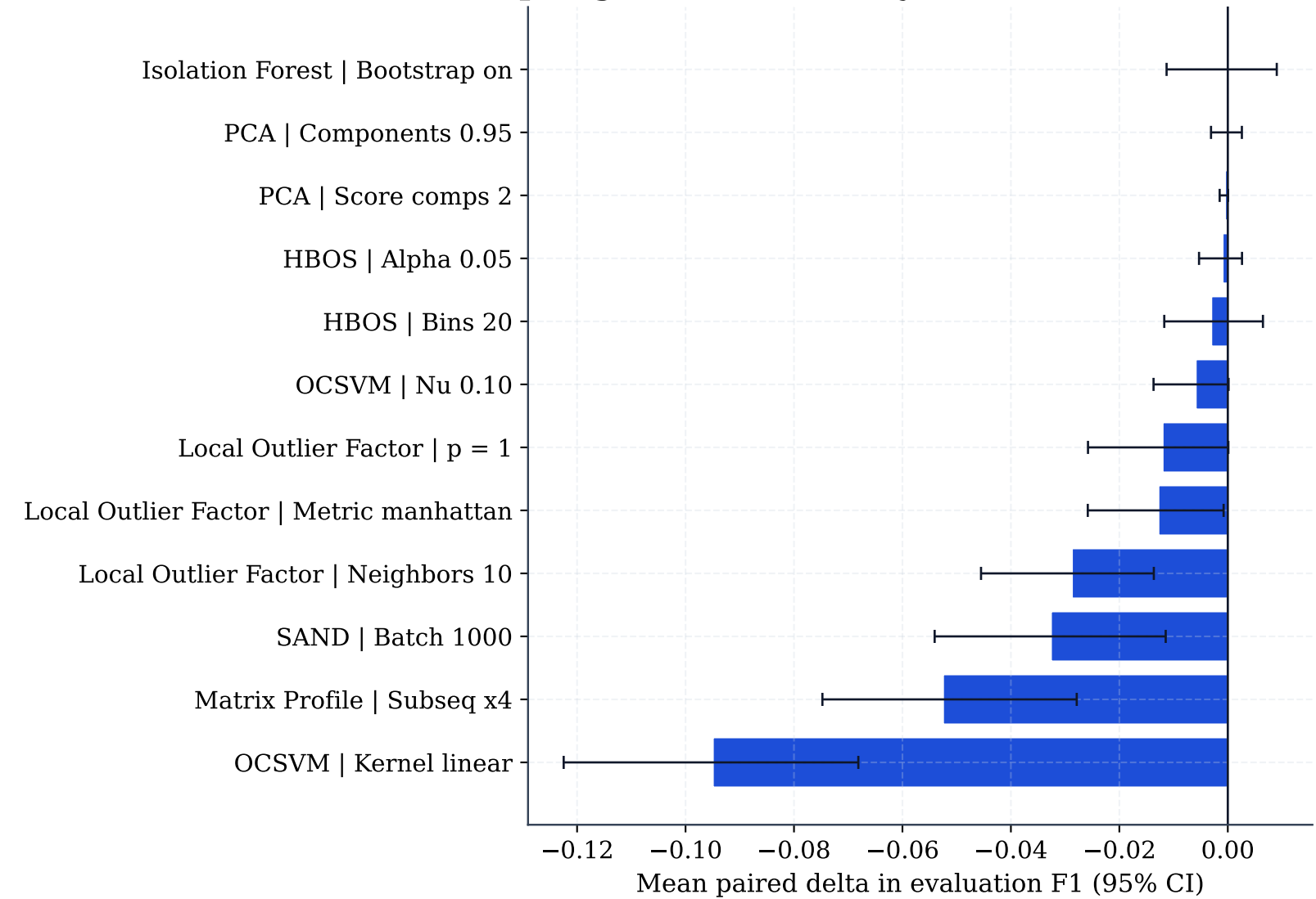
Best ablation per algorithm
