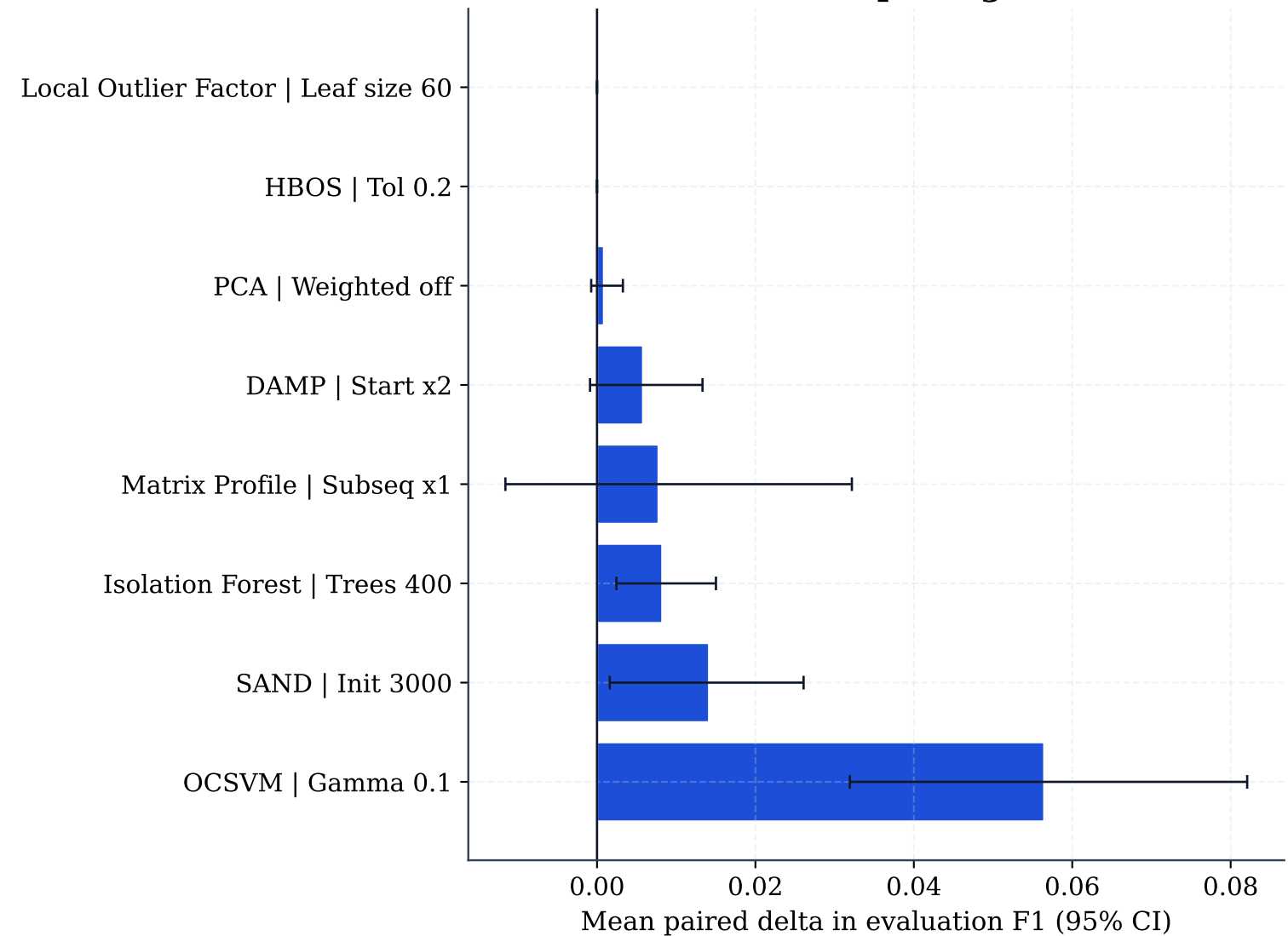
Best ablation per algorithm
