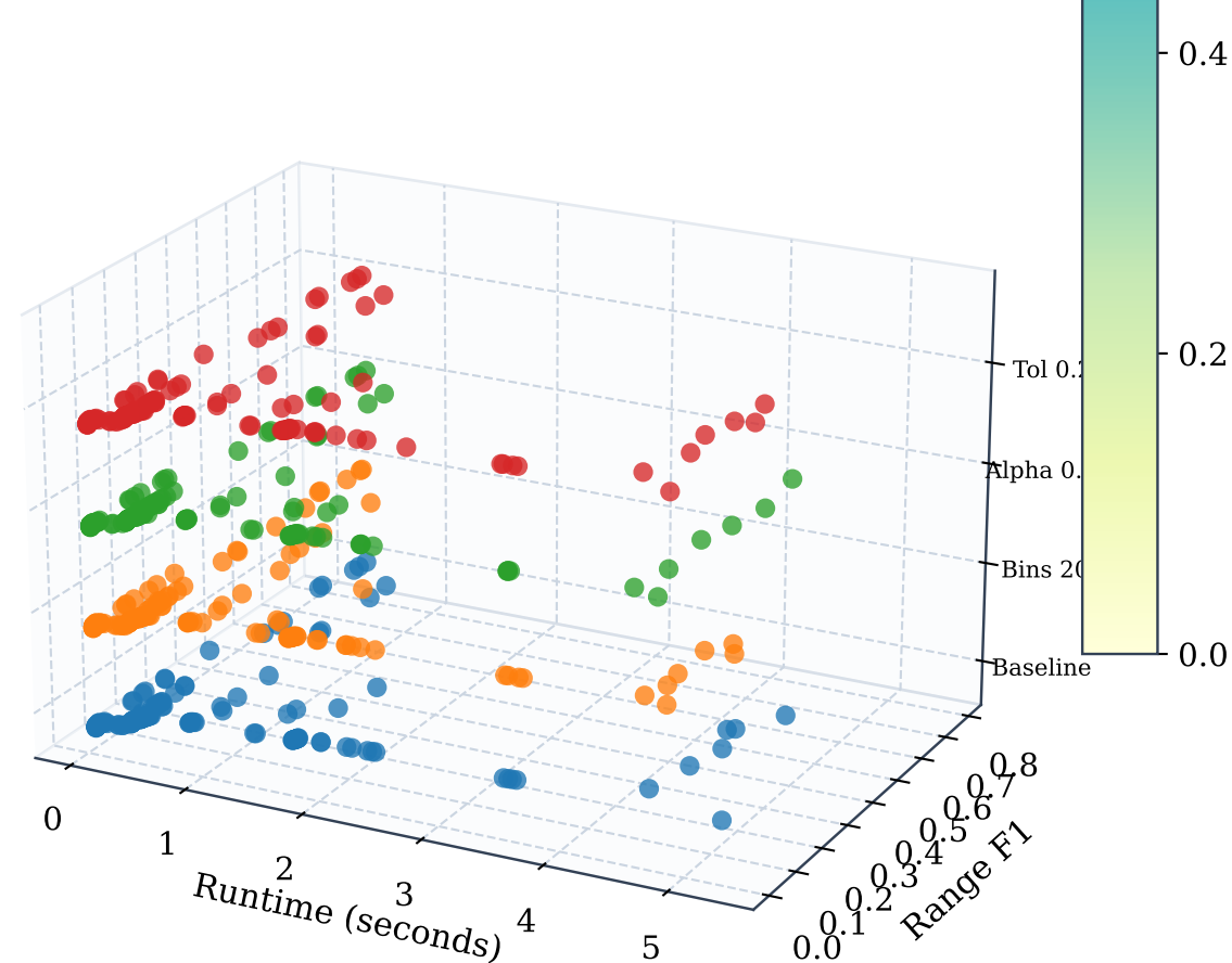
HBOS | Layered 3D runtime vs Range F1
