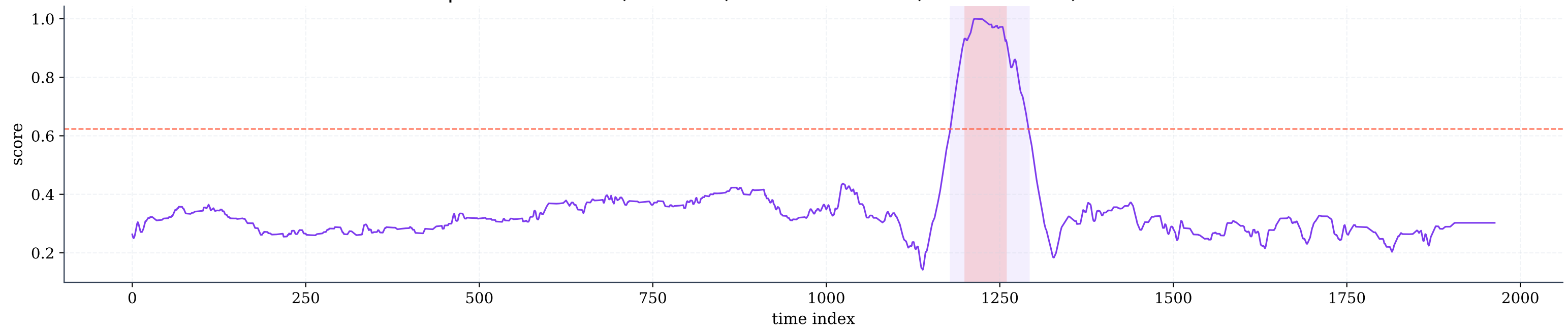
score | ROC AUC=1.00, F1=0.69, Eval Recall=1.00, Eval F1=0.69, runtime=0.27s
