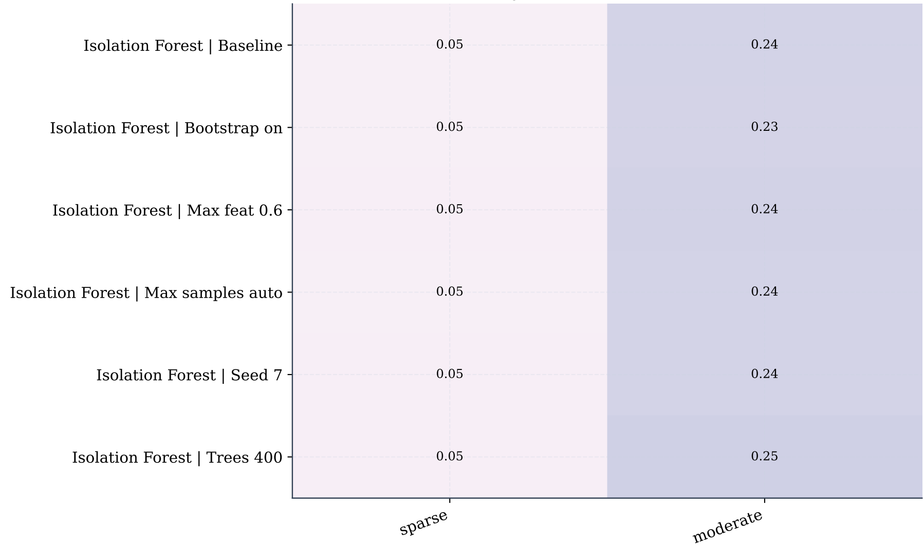
Isolation Forest | Mean Range F1 by anomaly ratio
