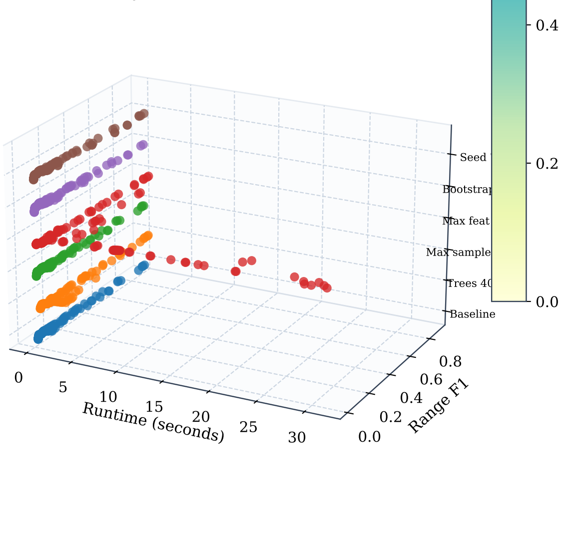
Isolation Forest | Layered 3D runtime vs Range F1
