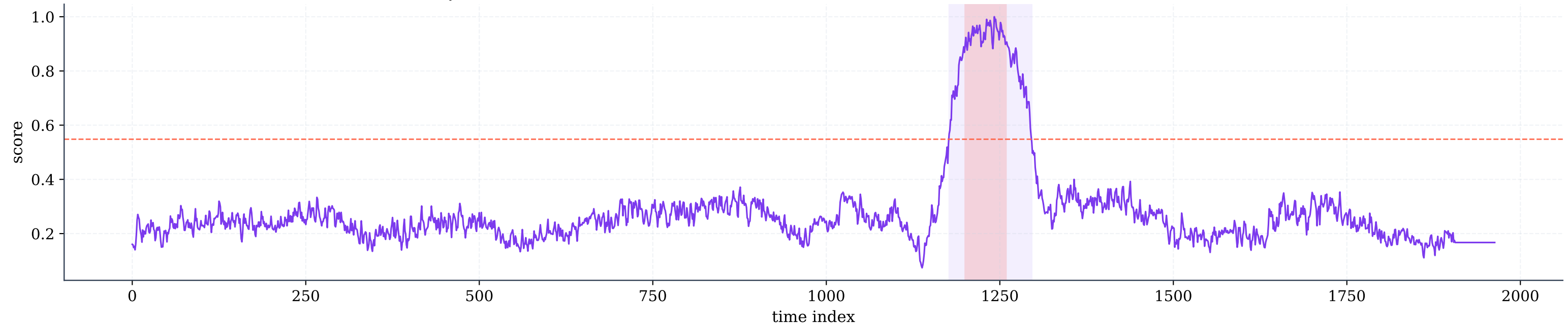
score | ROC AUC=1.00, F1=0.67, Eval Recall=1.00, Eval F1=0.67, runtime=0.37s
