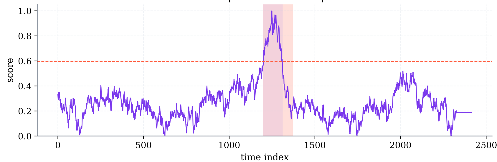
Variant 3: Max samples auto | Eval F1=0.83 | ROC AUC=0.91
