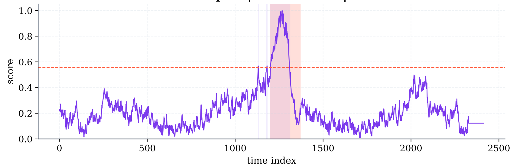
Variant 5: Bootstrap on | Eval F1=0.37 | ROC AUC=0.88
