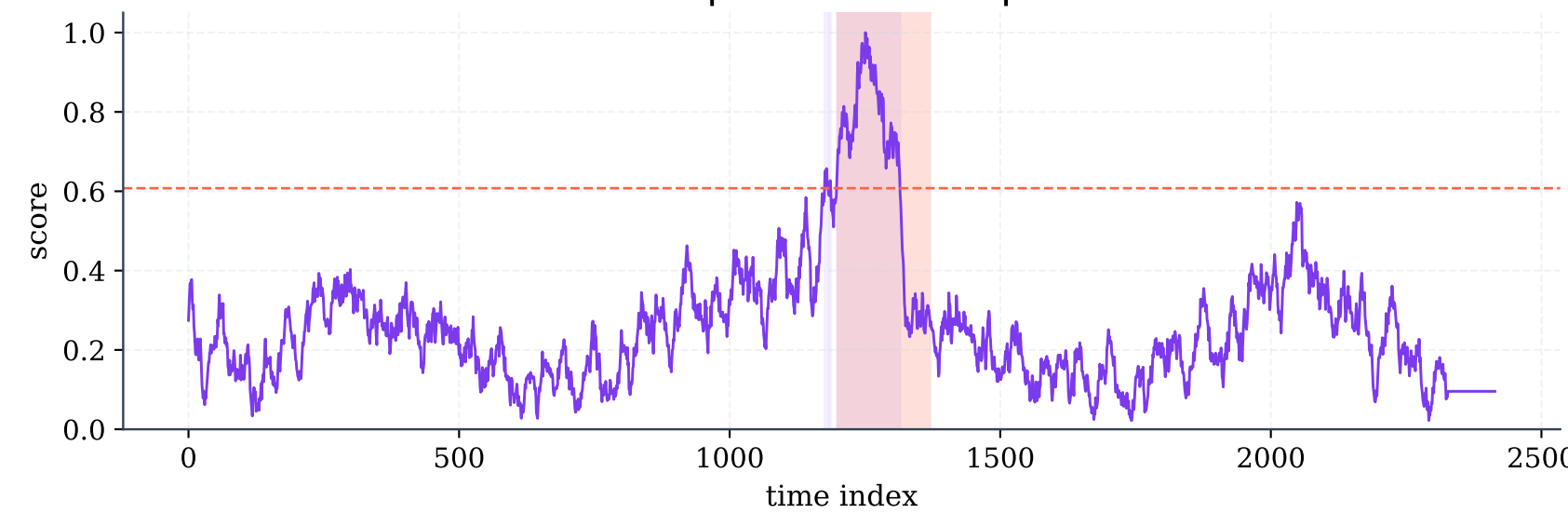
Variant 6: Seed 7 | Eval F1=0.46 | ROC AUC=0.92
