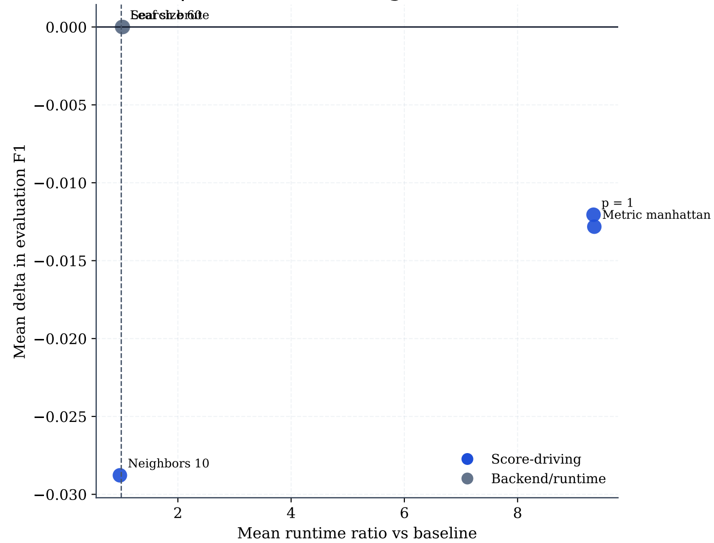
Local Outlier Factor | Runtime tradeoff against mean delta in evaluation F1
