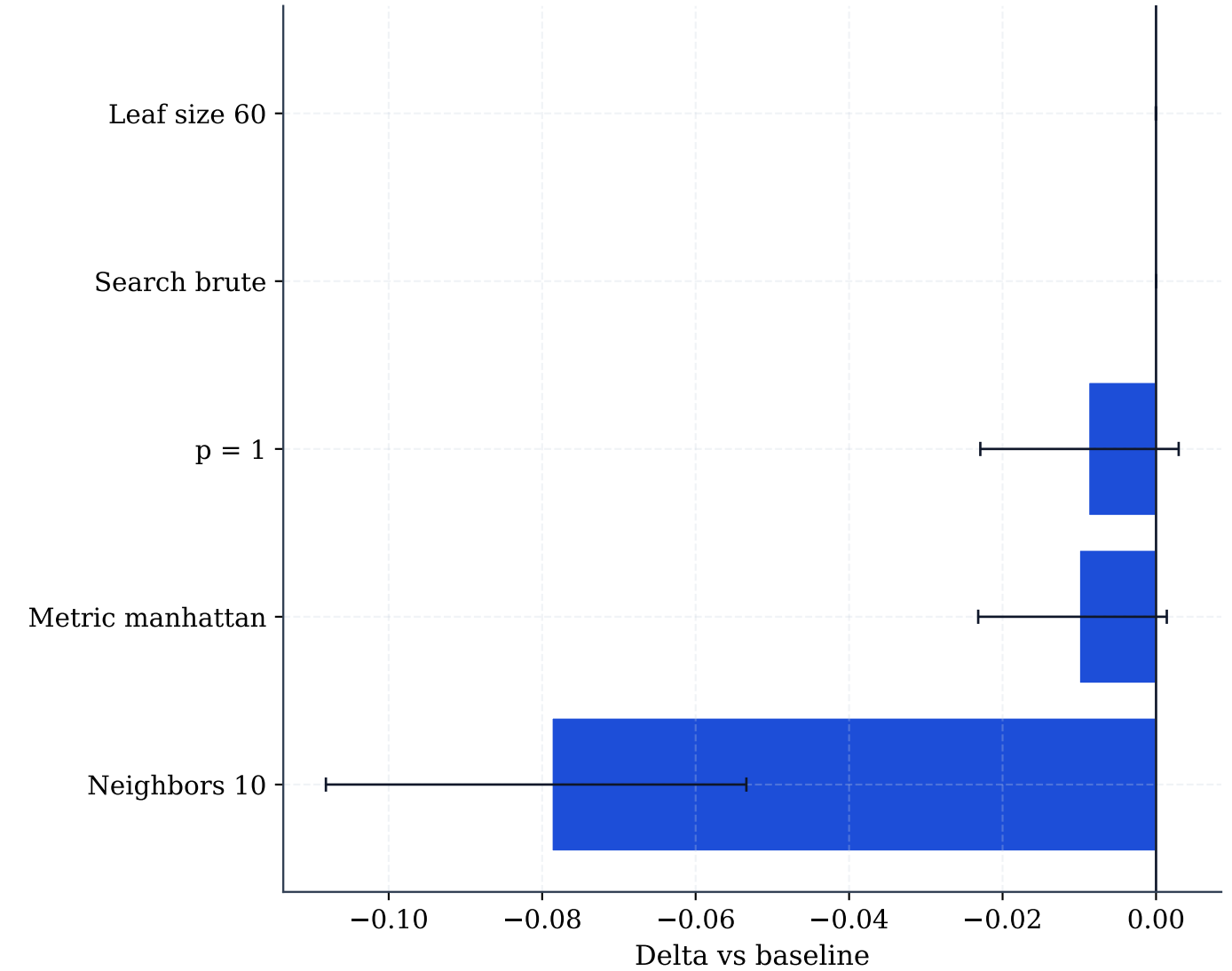
Local Outlier Factor | Mean paired delta in evaluation F1 by dataset variant
