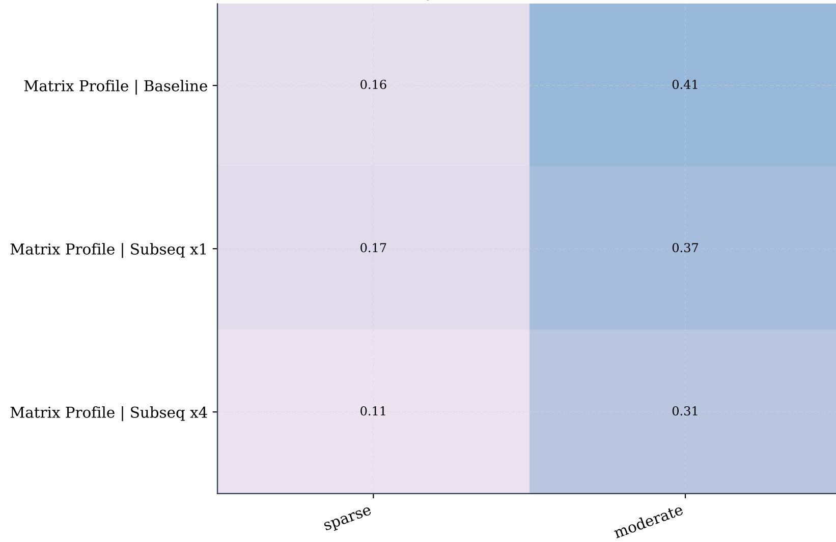
Matrix Profile | Mean Range F1 by anomaly ratio
