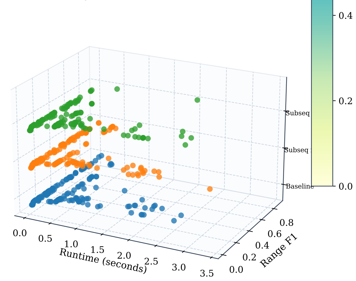
Matrix Profile | Layered 3D runtime vs Range F1
