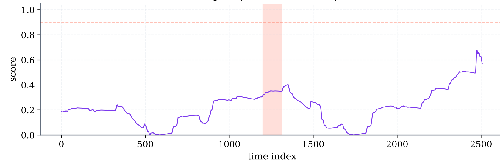
Variant 3: Subseq x4 | Eval F1=0.00 | ROC AUC=0.77
