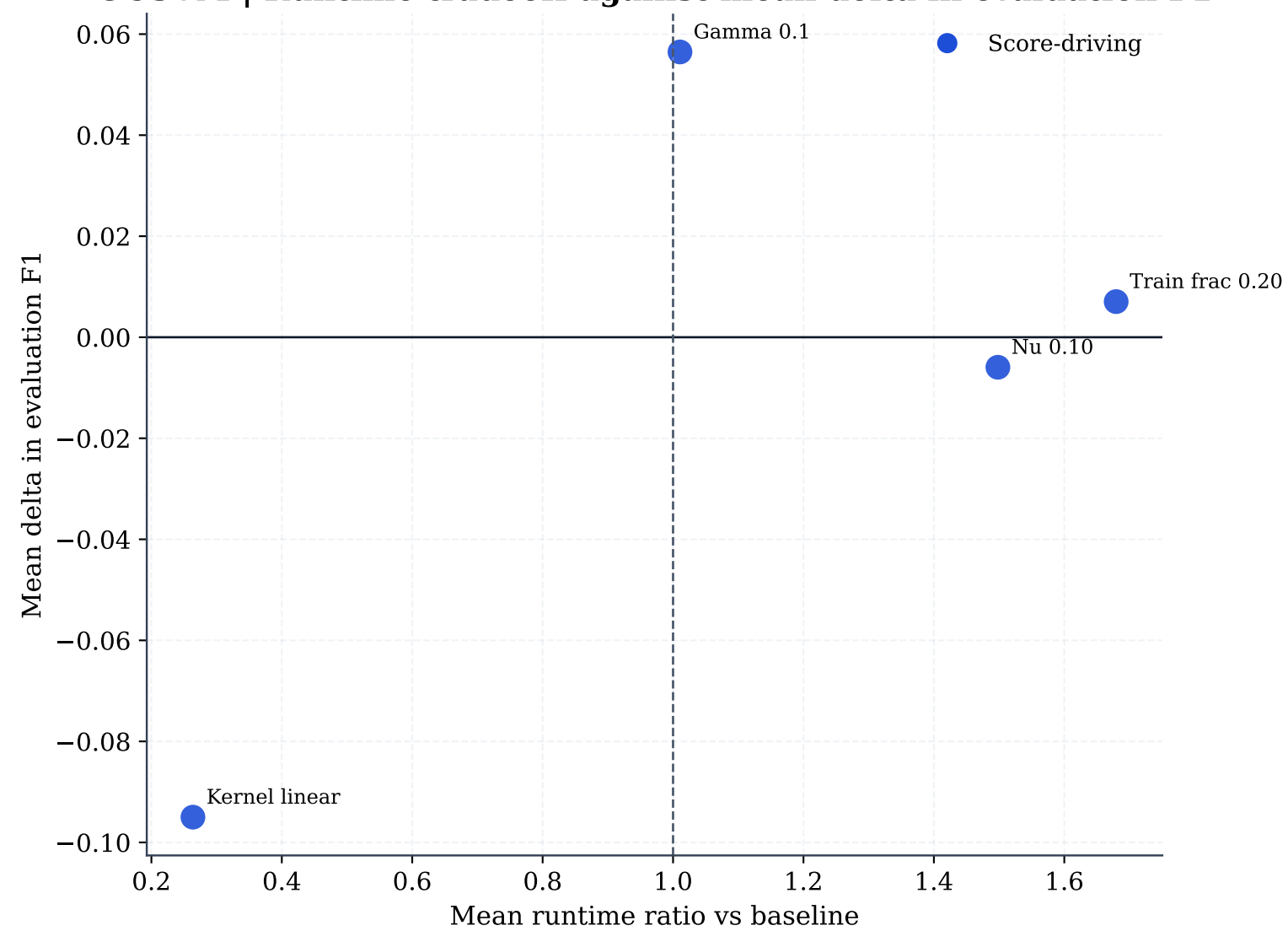
OCSVM | Runtime tradeoff against mean delta in evaluation F1
