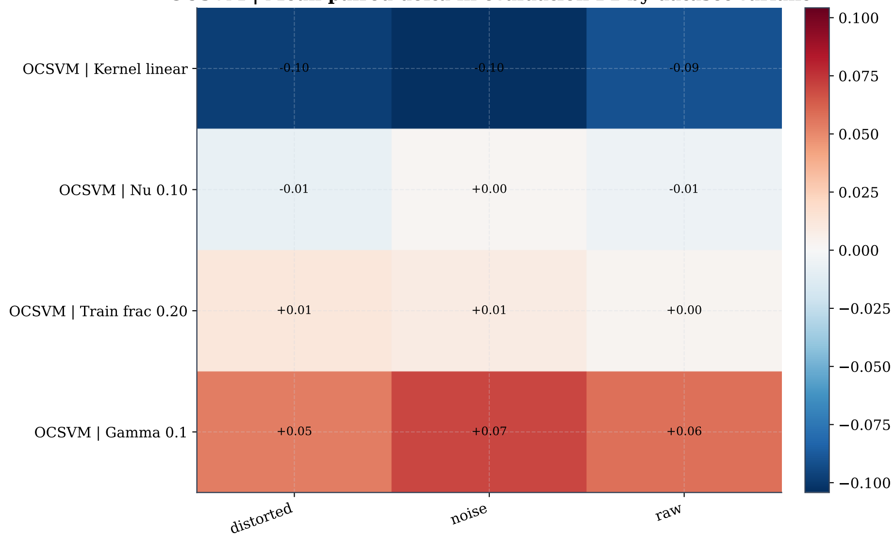
OCSVM | Mean paired delta in evaluation F1 by dataset variant
