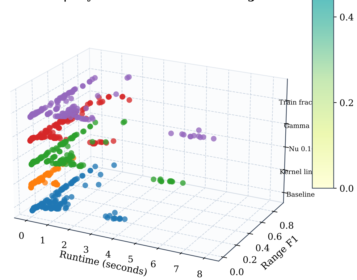
OCSVM | Layered 3D runtime vs Range F1
