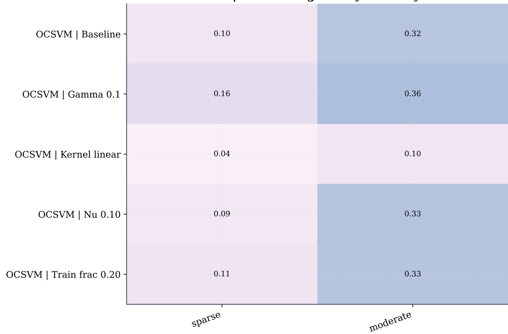
OCSVM | Mean Range F1 by anomaly ratio
