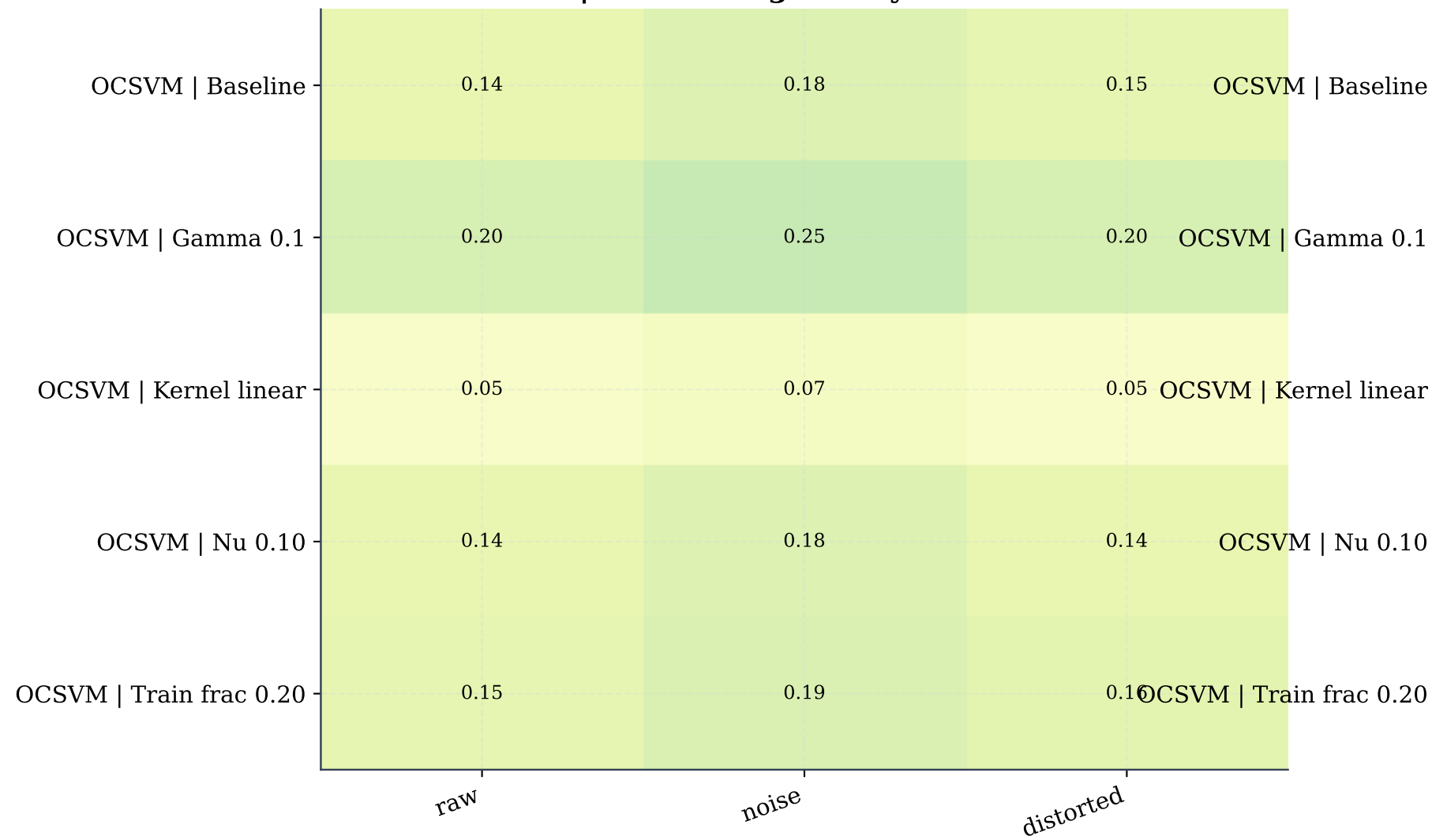
OCSVM | Mean Range F1 by dataset variant
